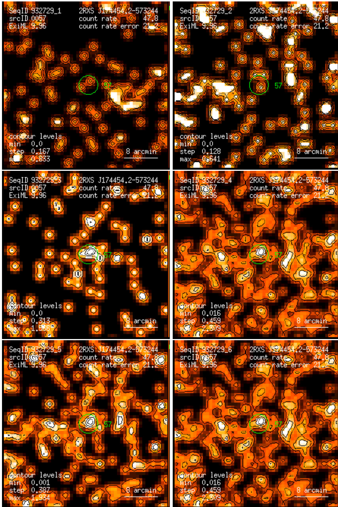
Figure 57: RASS 932729: detection 0057: band rate images, Gaussian filter: (1) PSPC channels 11 – 41, (2) 52 – 90, (3) 91 – 201, (4) 11 – 235, (5) 52 – 201, (6) 11 – 201. Broad band rates in counts/ks. Band rate contour levels in counts/ks/arcmin 2 .
