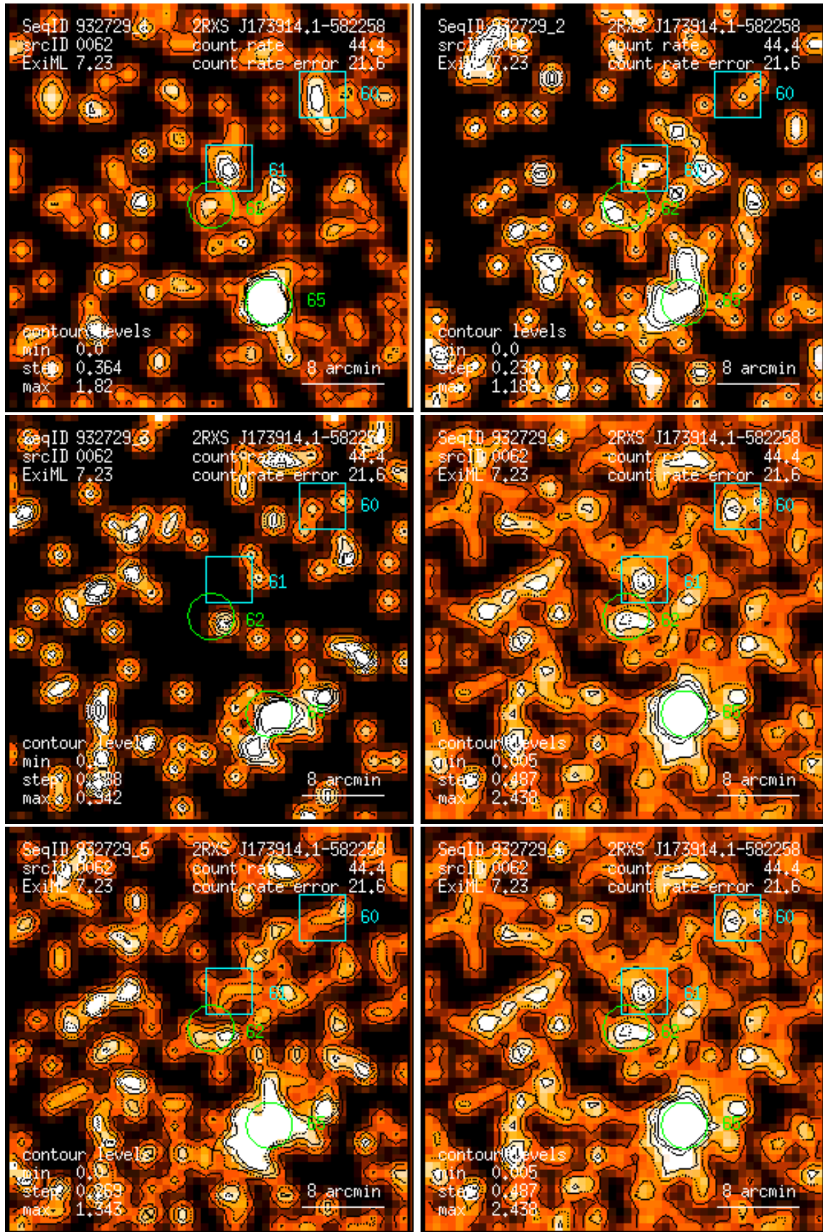
Figure 62: RASS 932729: detection 0062: band rate images, Gaussian filter: (1) PSPC channels 11 – 41, (2) 52 – 90, (3) 91 – 201, (4) 11 – 235, (5) 52 – 201, (6) 11 – 201. Broad band rates in counts/ks. Band rate contour levels in counts/ks/arcmin 2 .
