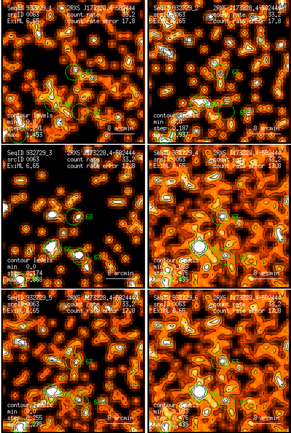
Figure 63: RASS 932729: detection 0063: band rate images, Gaussian filter: (1) PSPC channels 11 – 41, (2) 52 – 90, (3) 91 – 201, (4) 11 – 235, (5) 52 – 201, (6) 11 – 201. Broad band rates in counts/ks. Band rate contour levels in counts/ks/arcmin 2 .
