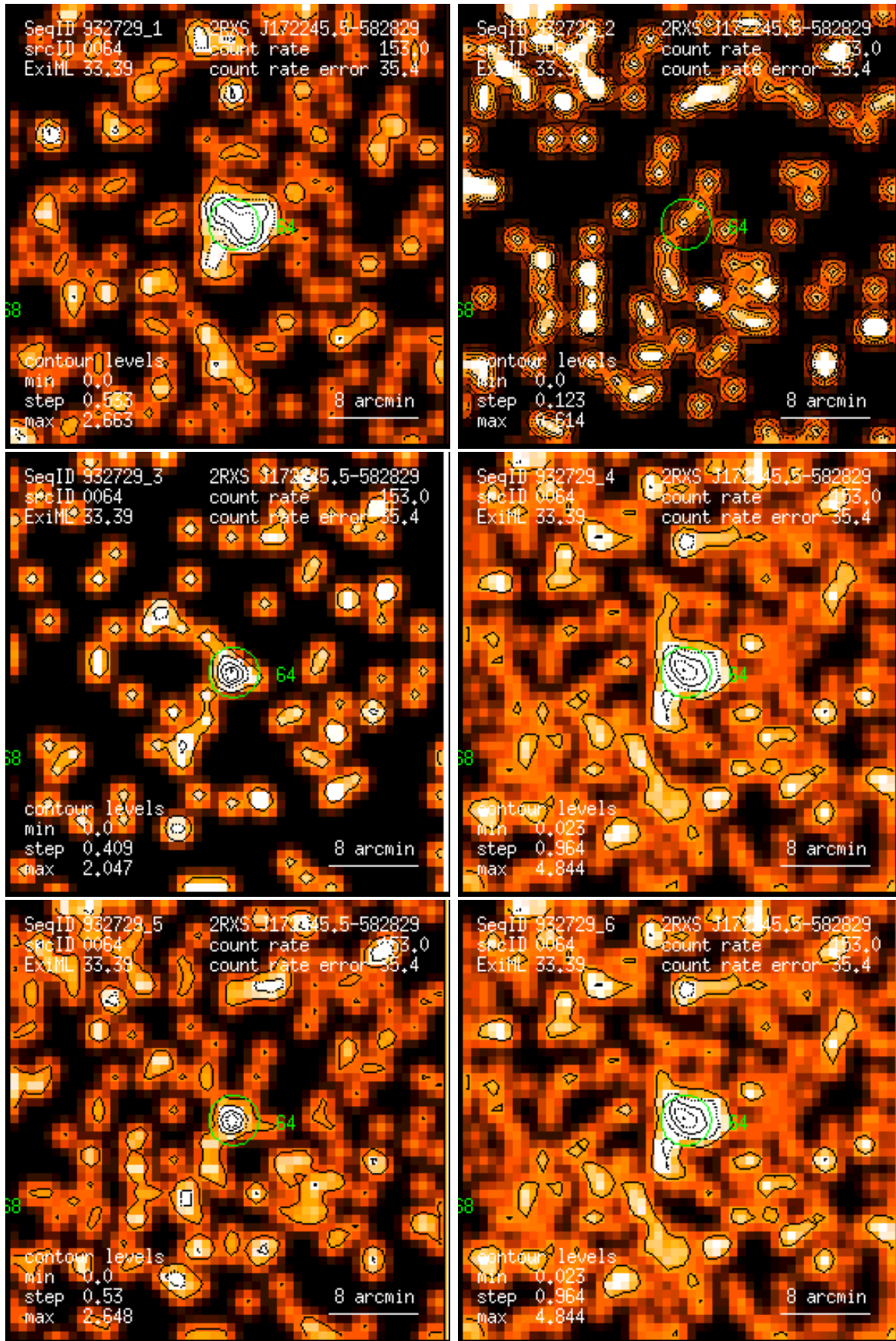
Figure 64: RASS 932729: detection 0064: band rate images, Gaussian filter: (1) PSPC channels 11 – 41, (2) 52 – 90, (3) 91 – 201, (4) 11 – 235, (5) 52 – 201, (6) 11 – 201. Broad band rates in counts/ks. Band rate contour levels in counts/ks/arcmin 2 .
