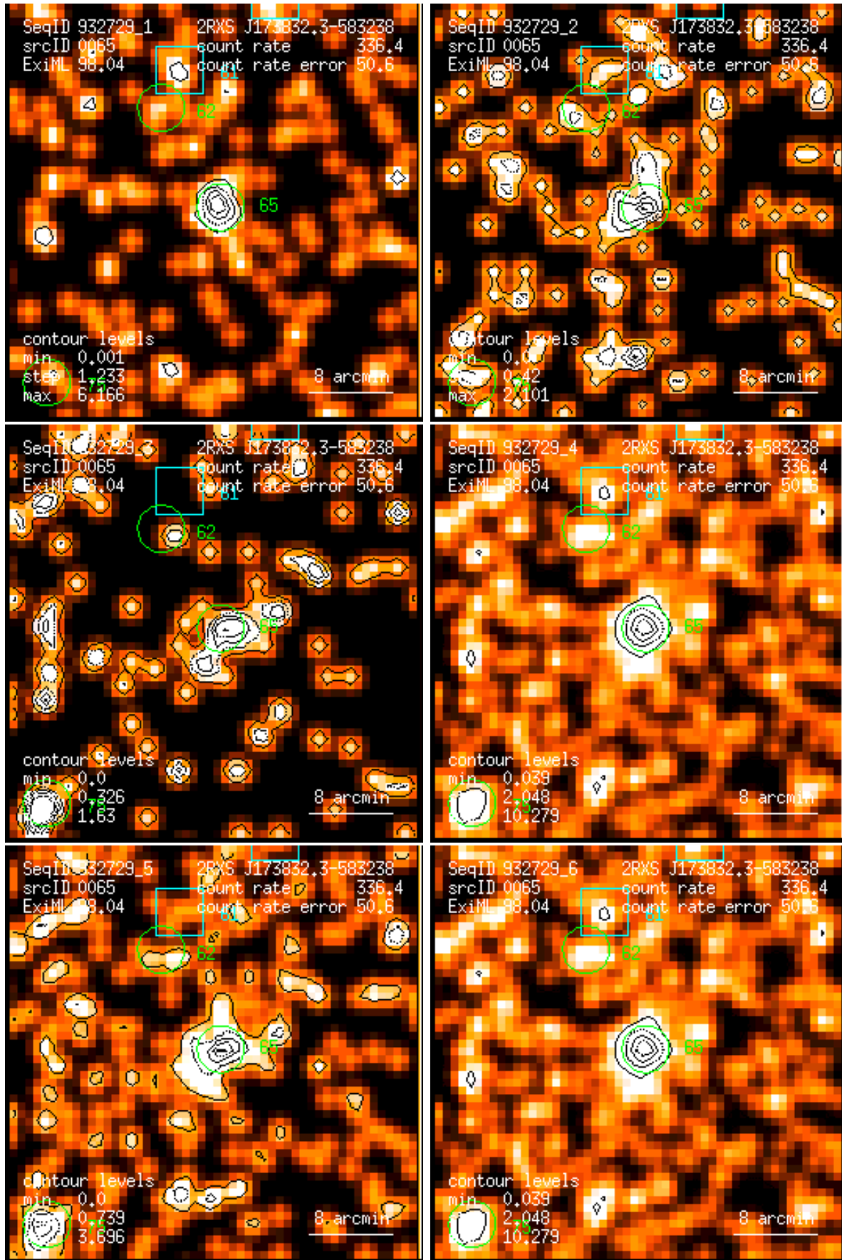
Figure 65: RASS 932729: detection 0065: band rate images, Gaussian filter: (1) PSPC channels 11 – 41, (2) 52 – 90, (3) 91 – 201, (4) 11 – 235, (5) 52 – 201, (6) 11 – 201. Broad band rates in counts/ks. Band rate contour levels in counts/ks/arcmin 2 .
