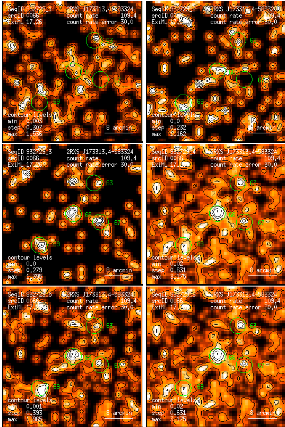
Figure 66: RASS 932729: detection 0066: band rate images, Gaussian filter: (1) PSPC channels 11 – 41, (2) 52 – 90, (3) 91 – 201, (4) 11 – 235, (5) 52 – 201, (6) 11 – 201. Broad band rates in counts/ks. Band rate contour levels in counts/ks/arcmin 2 .
