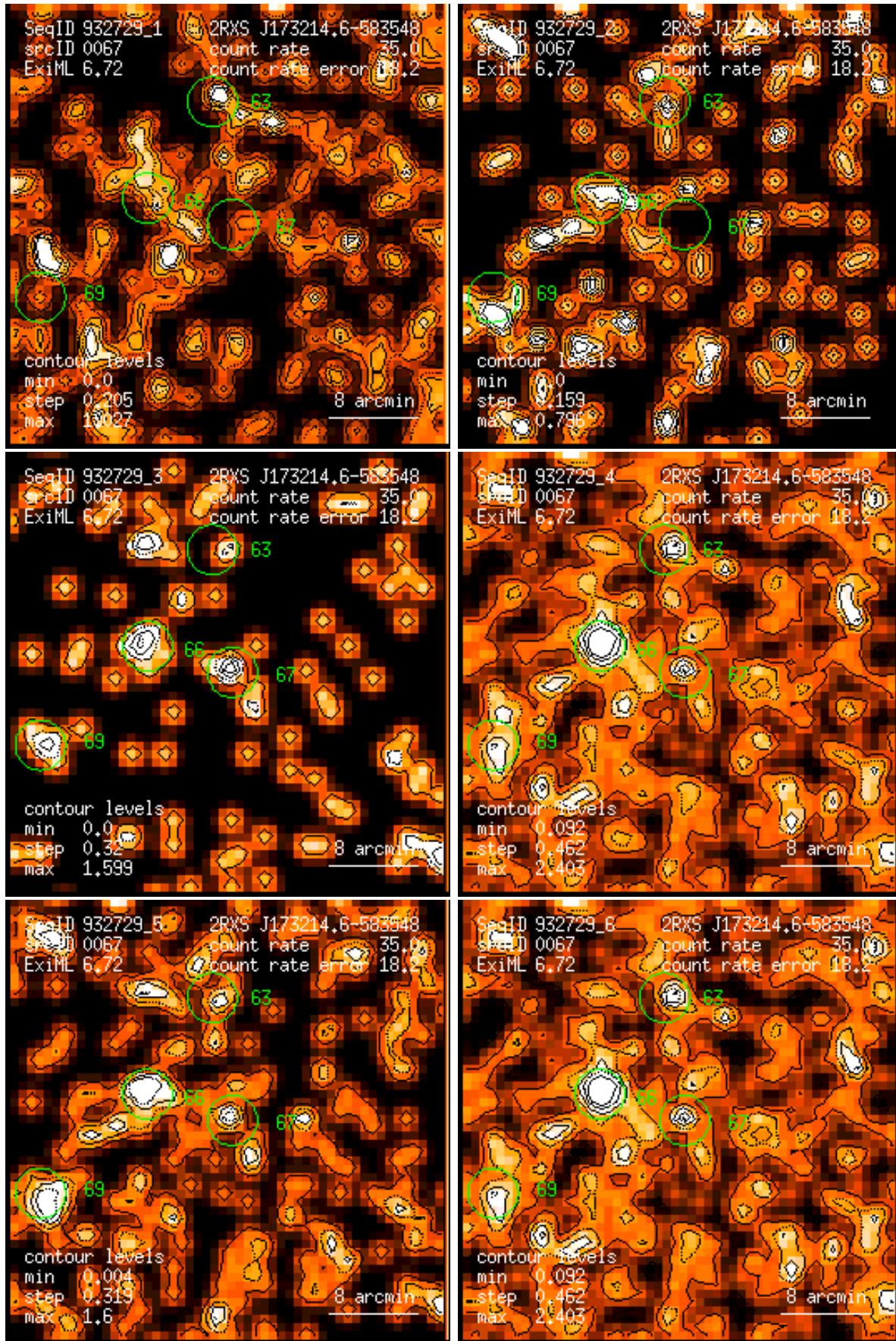
Figure 67: RASS 932729: detection 0067: band rate images, Gaussian filter: (1) PSPC channels 11 – 41, (2) 52 – 90, (3) 91 – 201, (4) 11 – 235, (5) 52 – 201, (6) 11 – 201. Broad band rates in counts/ks. Band rate contour levels in counts/ks/arcmin 2 .
