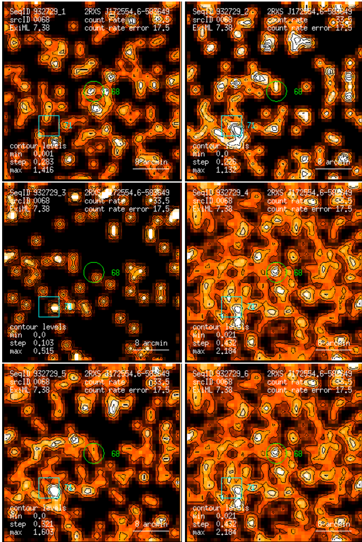
Figure 68: RASS 932729: detection 0068: band rate images, Gaussian filter: (1) PSPC channels 11 – 41, (2) 52 – 90, (3) 91 – 201, (4) 11 – 235, (5) 52 – 201, (6) 11 – 201. Broad band rates in counts/ks. Band rate contour levels in counts/ks/arcmin 2 .
