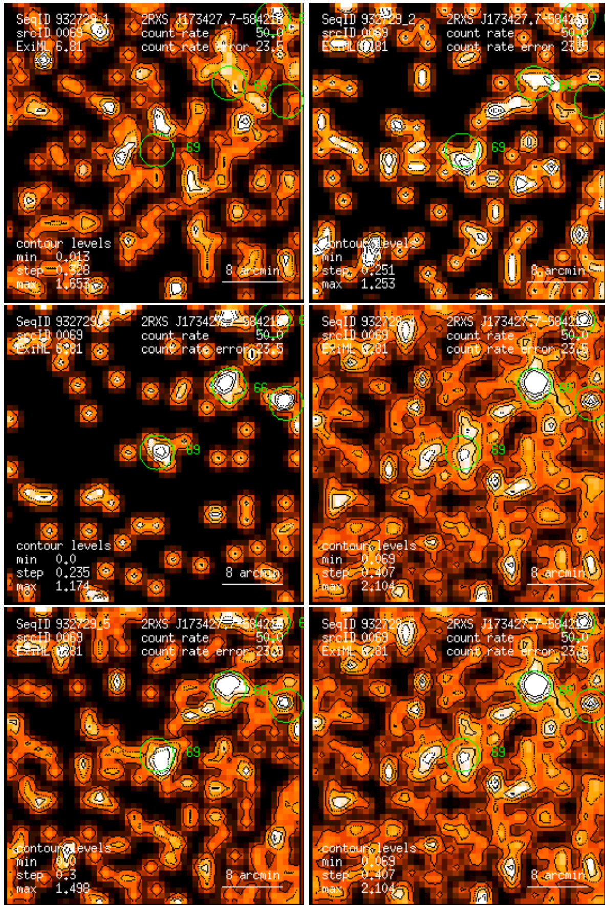
Figure 69: RASS 932729: detection 0069: band rate images, Gaussian filter: (1) PSPC channels 11 – 41, (2) 52 – 90, (3) 91 – 201, (4) 11 – 235, (5) 52 – 201, (6) 11 – 201. Broad band rates in counts/ks. Band rate contour levels in counts/ks/arcmin 2 .
