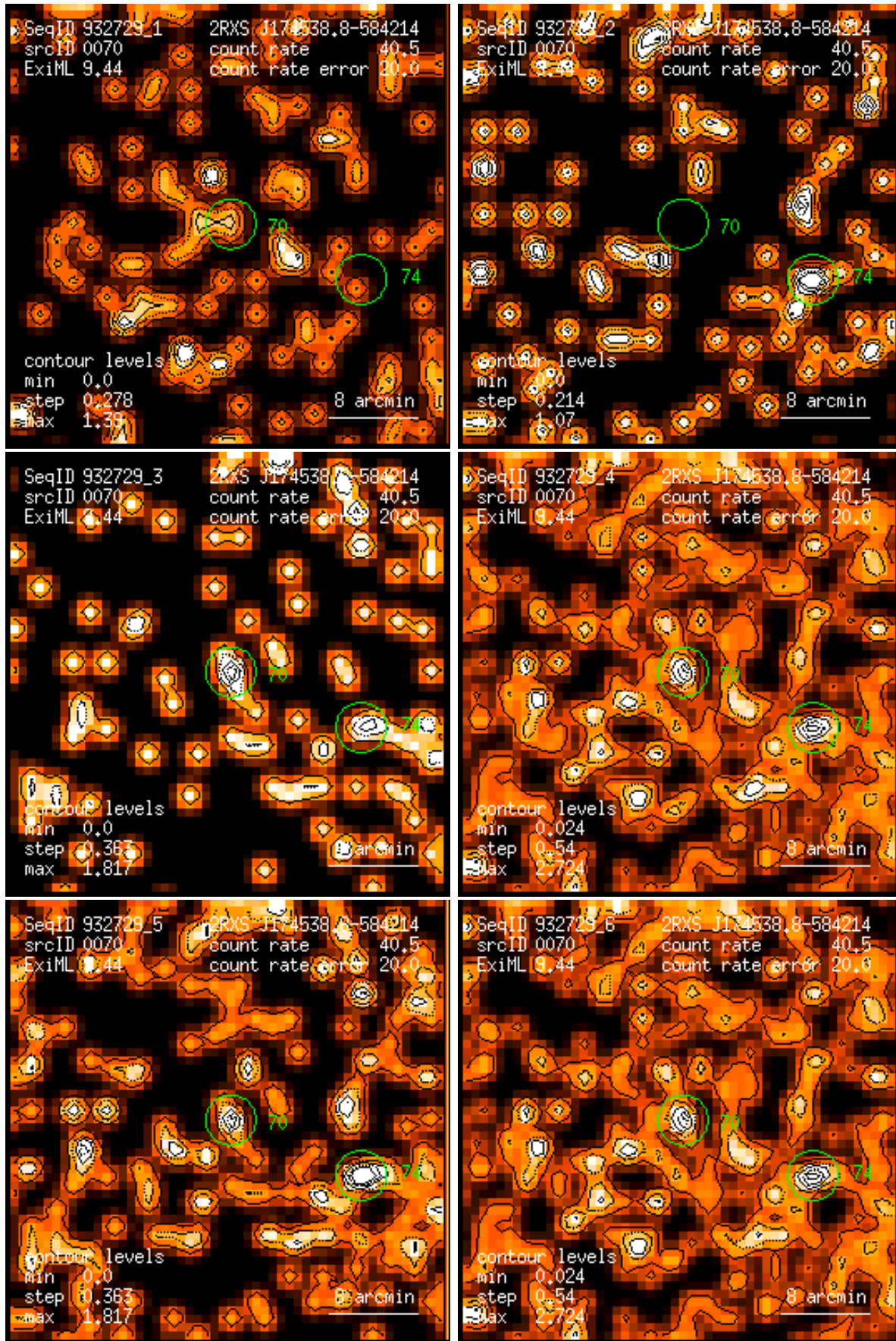
Figure 70: RASS 932729: detection 0070: band rate images, Gaussian filter: (1) PSPC channels 11 – 41, (2) 52 – 90, (3) 91 – 201, (4) 11 – 235, (5) 52 – 201, (6) 11 – 201. Broad band rates in counts/ks. Band rate contour levels in counts/ks/arcmin 2 .
