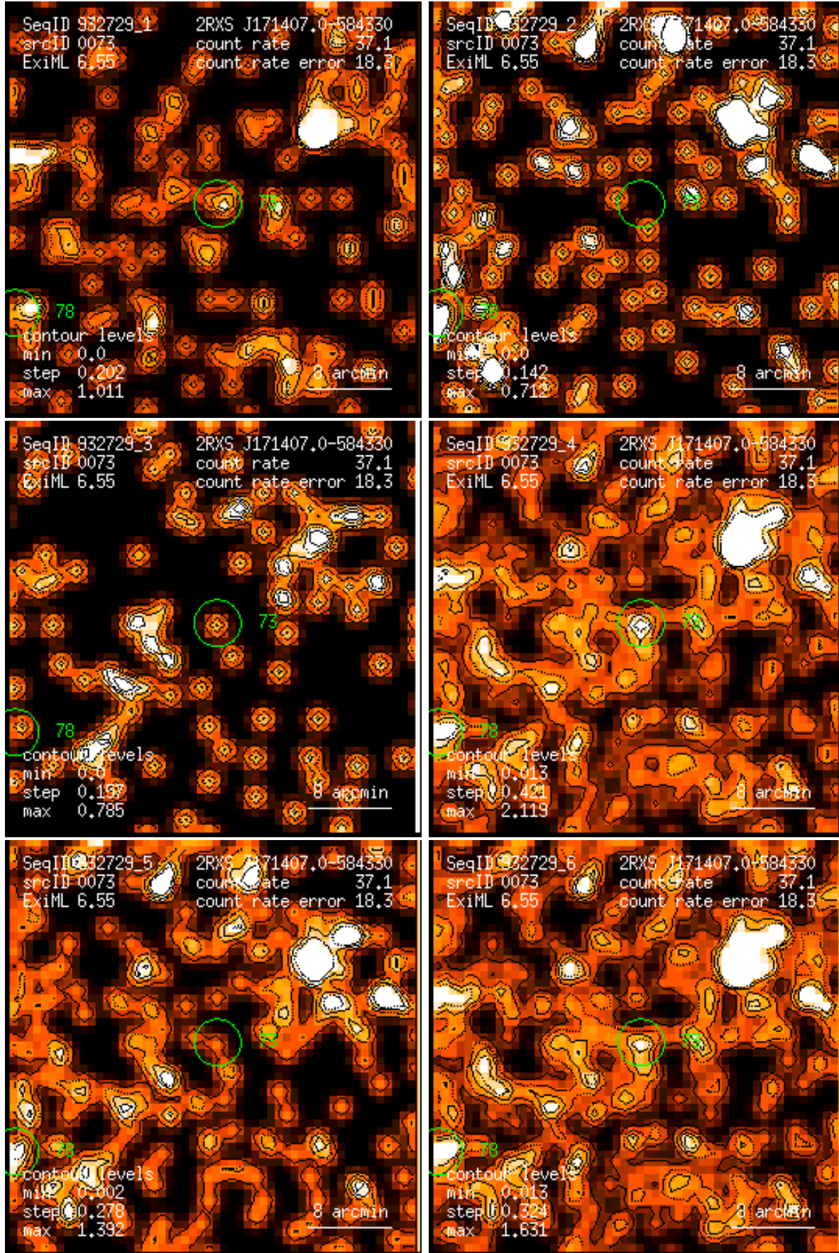
Figure 73: RASS 932729: detection 0073: band rate images, Gaussian filter: (1) PSPC channels 11 – 41, (2) 52 – 90, (3) 91 – 201, (4) 11 – 235, (5) 52 – 201, (6) 11 – 201. Broad band rates in counts/ks. Band rate contour levels in counts/ks/arcmin 2 .
