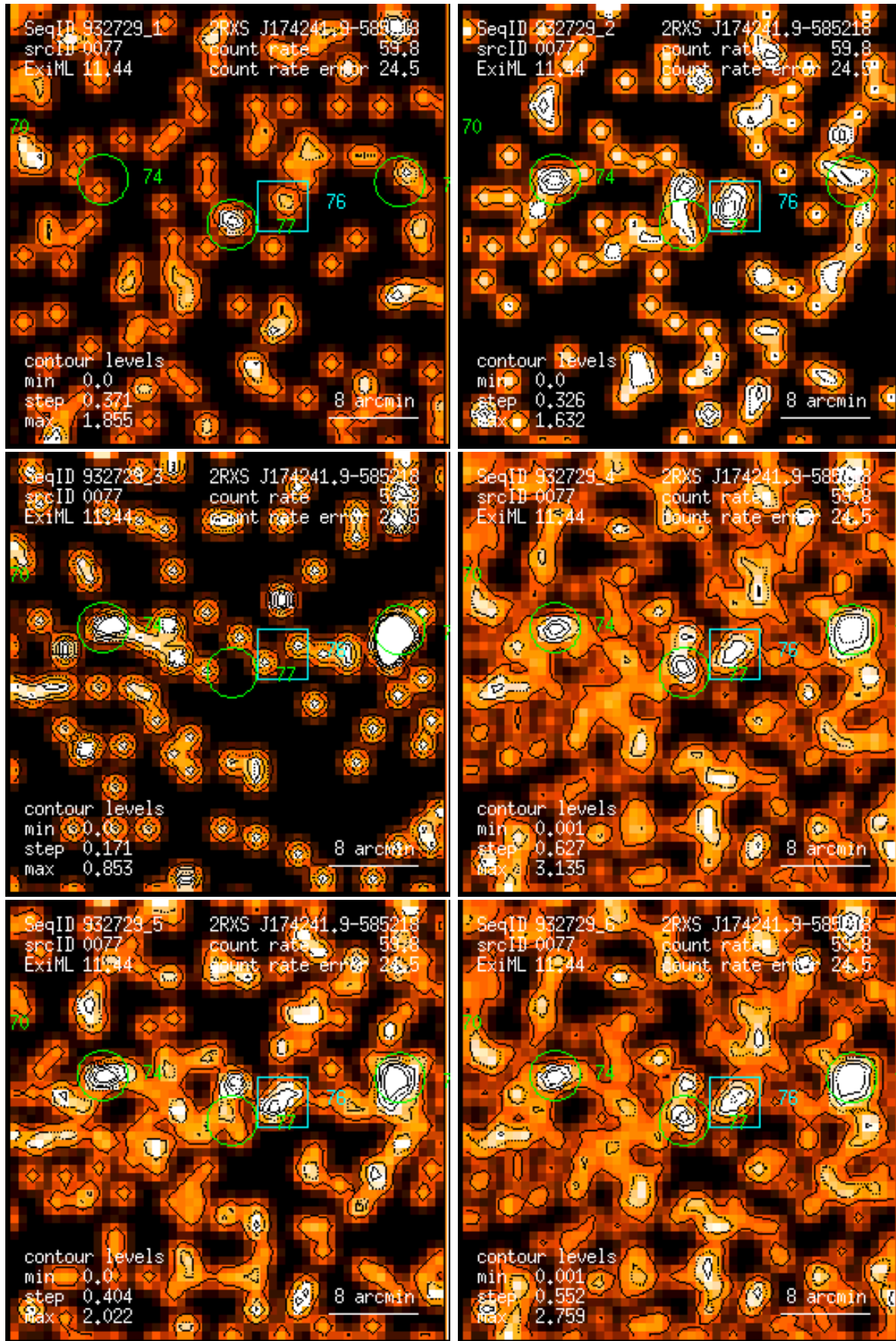
Figure 77: RASS 932729: detection 0077: band rate images, Gaussian filter: (1) PSPC channels 11 – 41, (2) 52 – 90, (3) 91 – 201, (4) 11 – 235, (5) 52 – 201, (6) 11 – 201. Broad band rates in counts/ks. Band rate contour levels in counts/ks/arcmin 2 .
