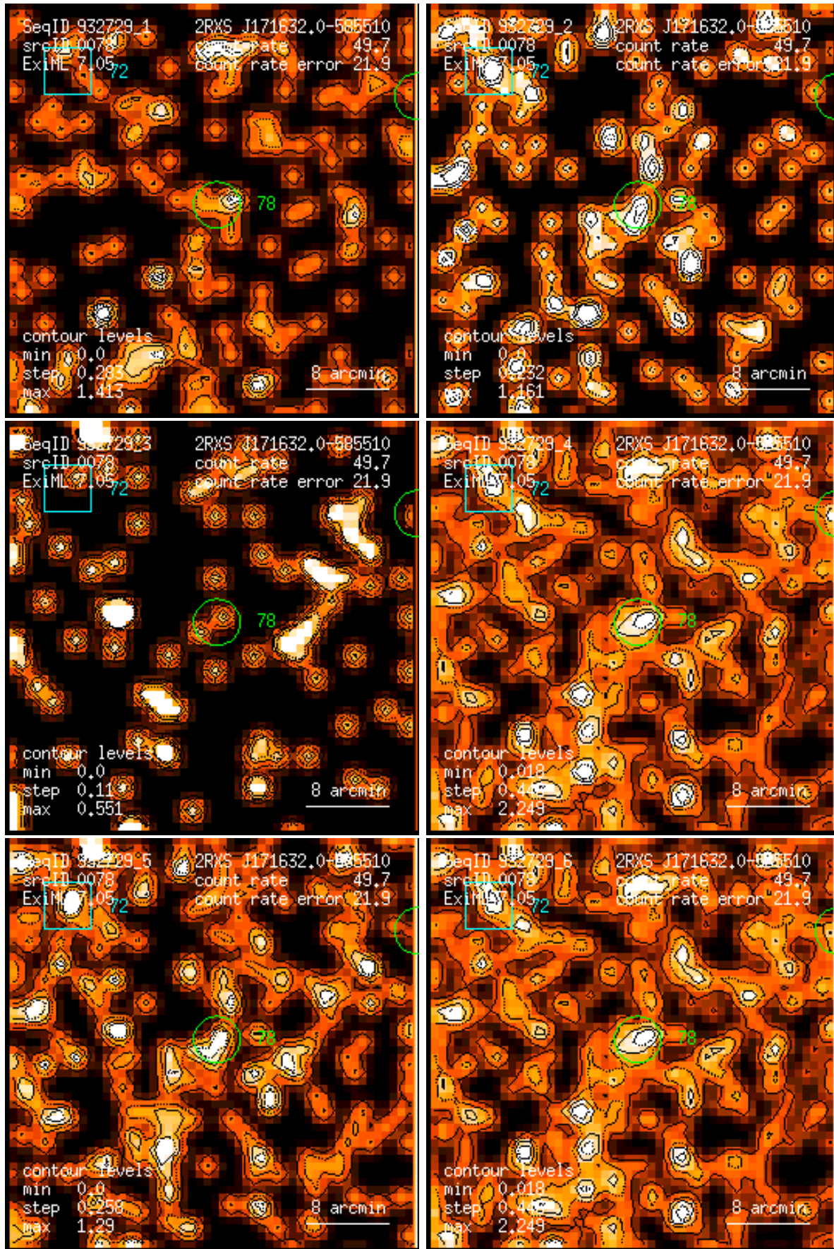
Figure 78: RASS 932729: detection 0078: band rate images, Gaussian filter: (1) PSPC channels 11 – 41, (2) 52 – 90, (3) 91 – 201, (4) 11 – 235, (5) 52 – 201, (6) 11 – 201. Broad band rates in counts/ks. Band rate contour levels in counts/ks/arcmin 2 .
