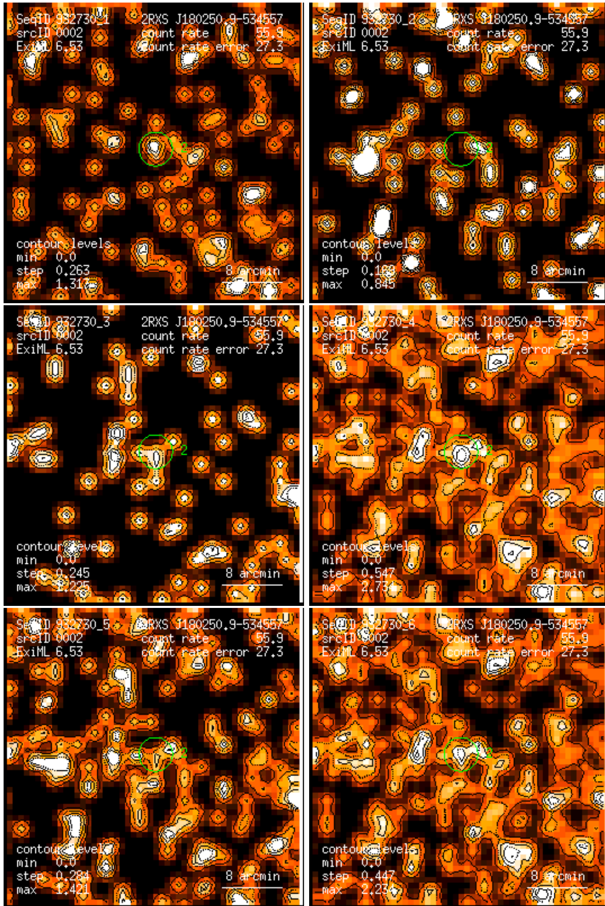
Figure 2: RASS 932730: detection 0002: band rate images, Gaussian filter: (1) PSPC channels 11 – 41, (2) 52 – 90, (3) 91 – 201, (4) 11 – 235, (5) 52 – 201, (6) 11 – 201. Broad band rates in counts/ks. Band rate contour levels in counts/ks/arcmin 2 .
