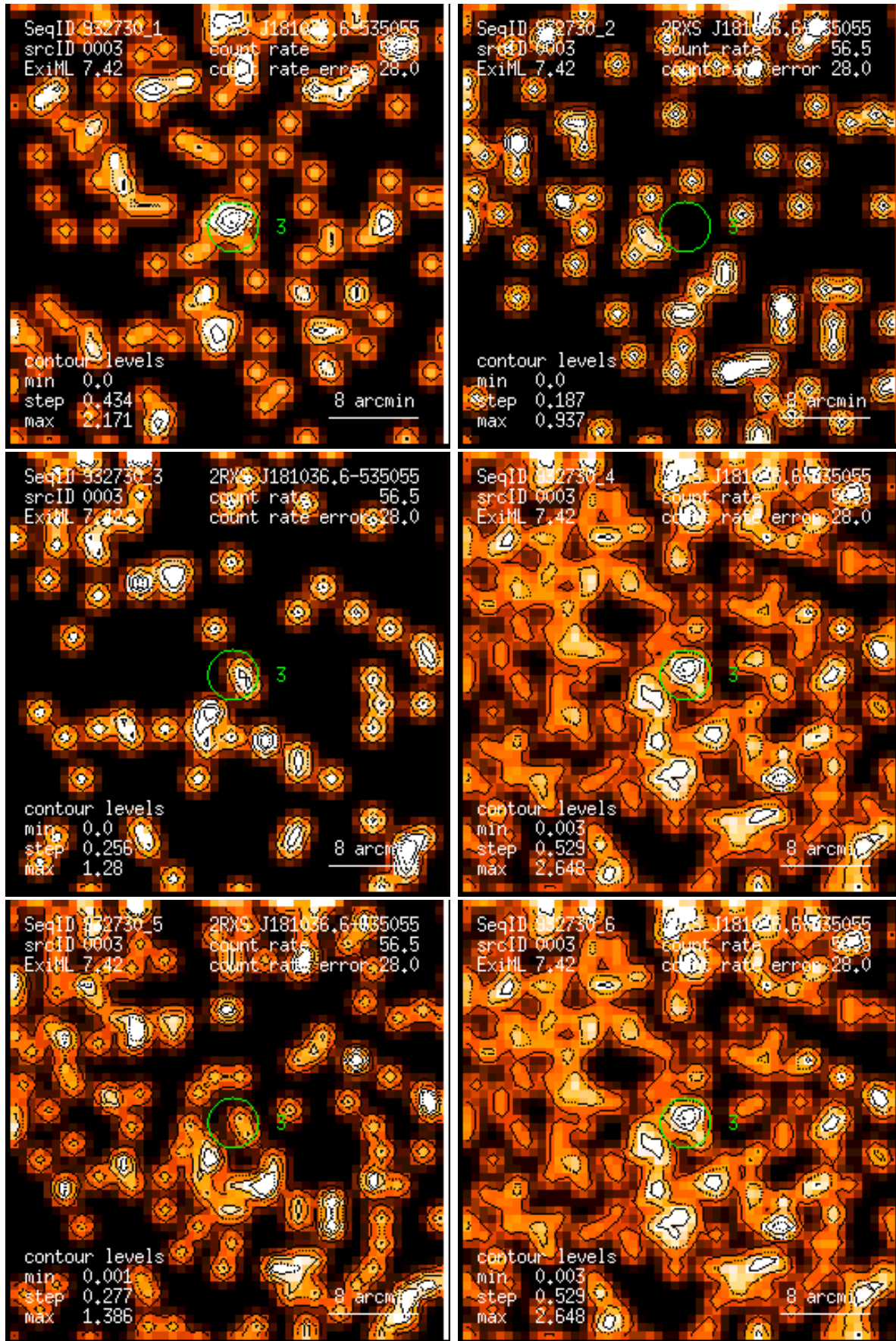
Figure 3: RASS 932730: detection 0003: band rate images, Gaussian filter: (1) PSPC channels 11 – 41, (2) 52 – 90, (3) 91 – 201, (4) 11 – 235, (5) 52 – 201, (6) 11 – 201. Broad band rates in counts/ks. Band rate contour levels in counts/ks/arcmin 2 .
