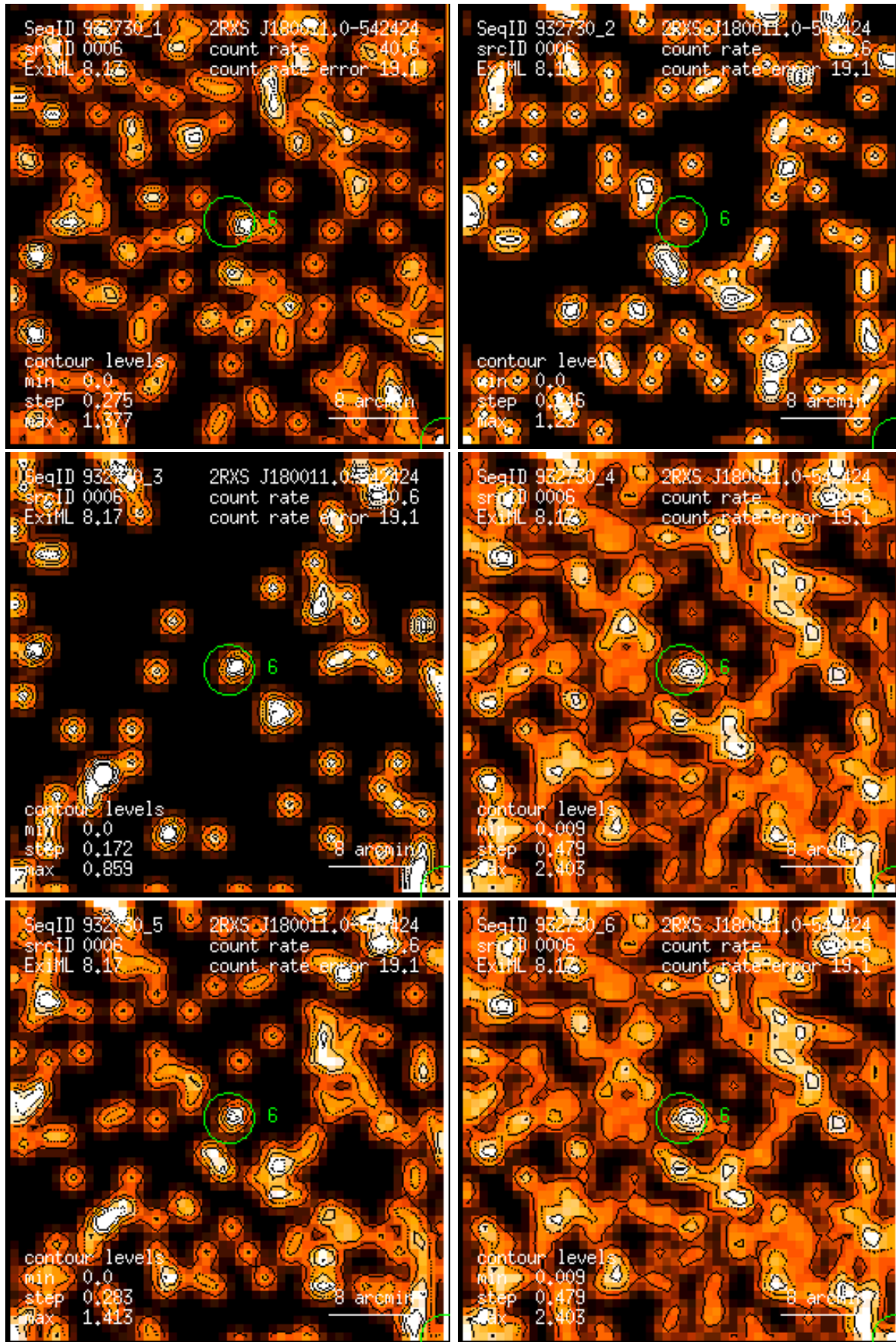
Figure 6: RASS 932730: detection 0006: band rate images, Gaussian filter: (1) PSPC channels 11 – 41, (2) 52 – 90, (3) 91 – 201, (4) 11 – 235, (5) 52 – 201, (6) 11 – 201. Broad band rates in counts/ks. Band rate contour levels in counts/ks/arcmin 2 .
