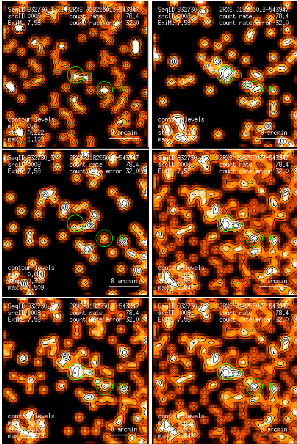
Figure 8: RASS 932730: detection 0008: band rate images, Gaussian filter: (1) PSPC channels 11 – 41, (2) 52 – 90, (3) 91 – 201, (4) 11 – 235, (5) 52 – 201, (6) 11 – 201. Broad band rates in counts/ks. Band rate contour levels in counts/ks/arcmin 2 .
