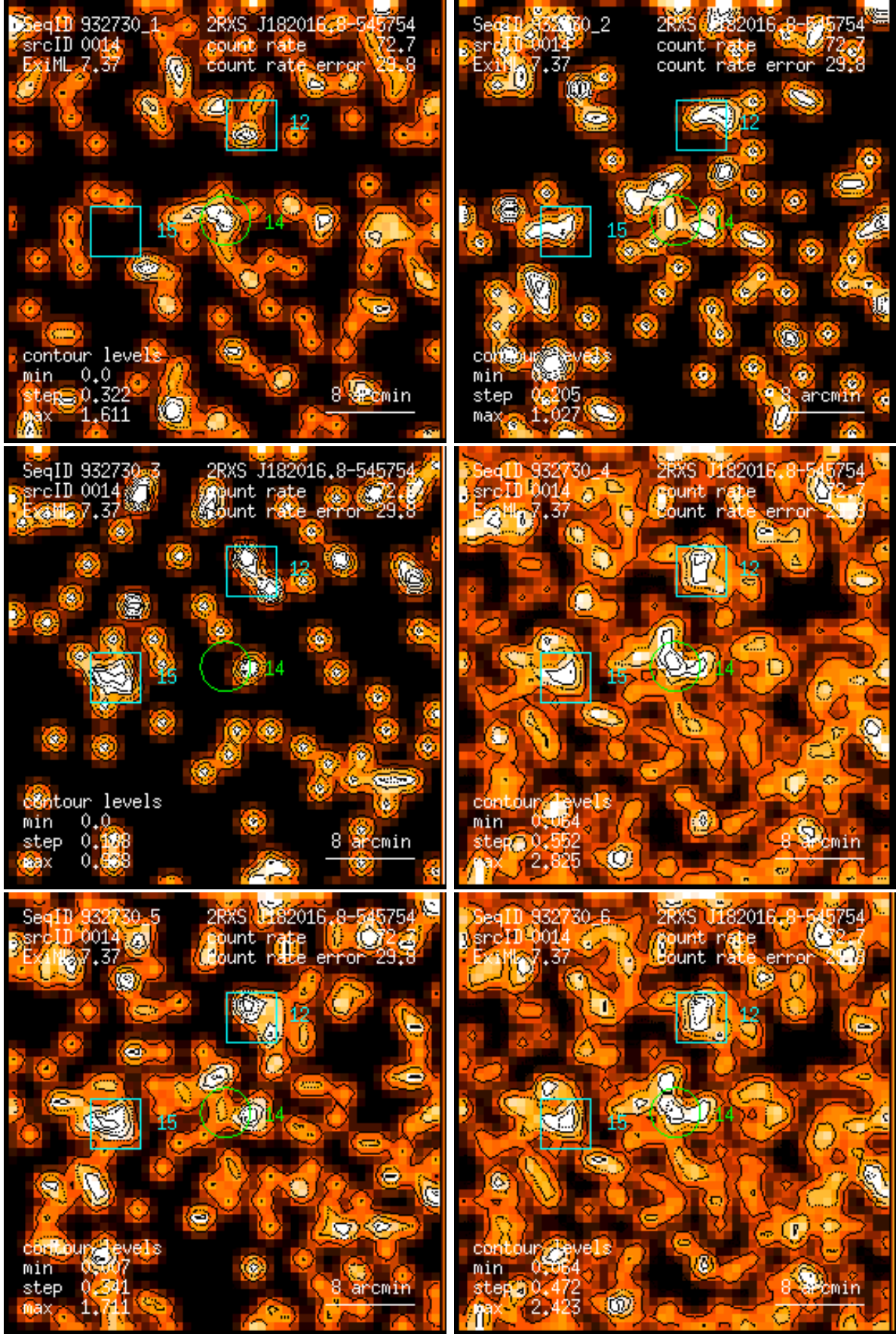
Figure 14: RASS 932730: detection 0014: band rate images, Gaussian filter: (1) PSPC channels 11 – 41, (2) 52 – 90, (3) 91 – 201, (4) 11 – 235, (5) 52 – 201, (6) 11 – 201. Broad band rates in counts/ks. Band rate contour levels in counts/ks/arcmin 2 .
