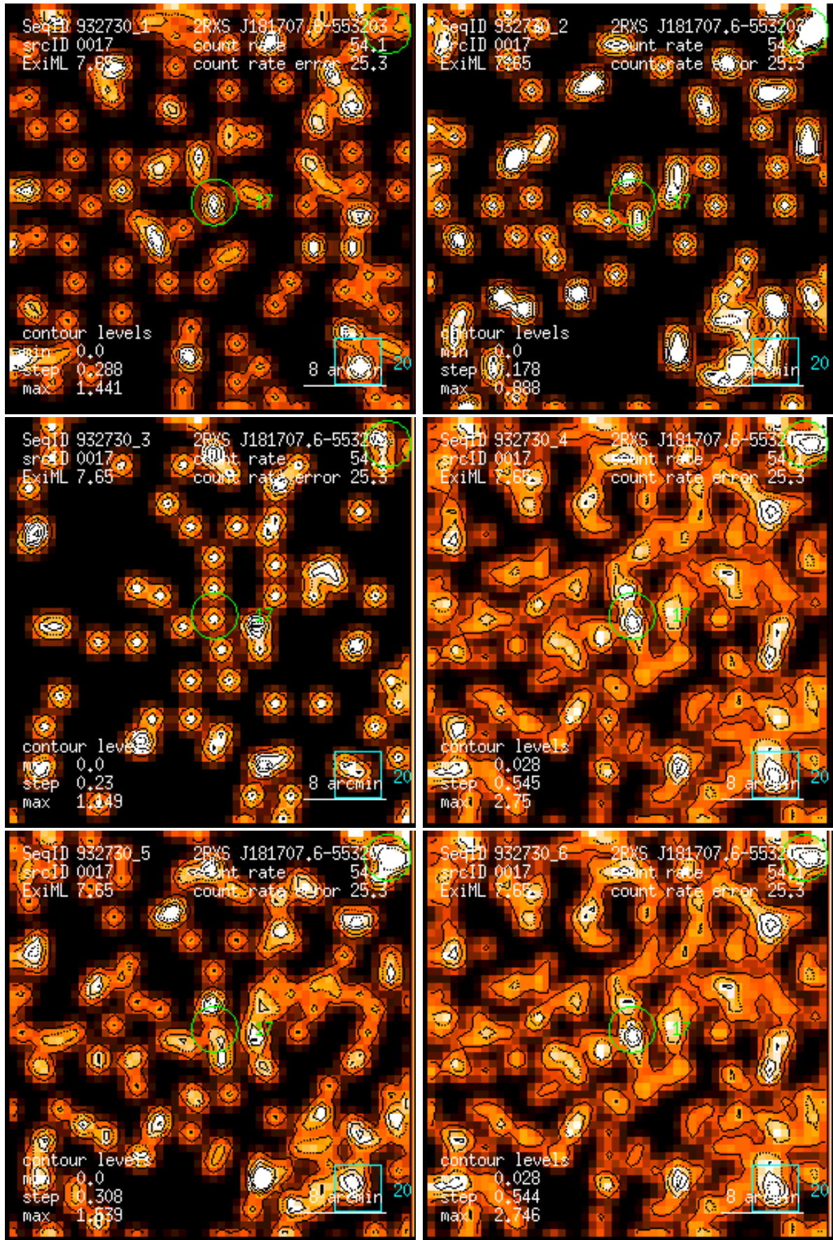
Figure 17: RASS 932730: detection 0017: band rate images, Gaussian filter: (1) PSPC channels 11 – 41, (2) 52 – 90, (3) 91 – 201, (4) 11 – 235, (5) 52 – 201, (6) 11 – 201. Broad band rates in counts/ks. Band rate contour levels in counts/ks/arcmin 2 .
