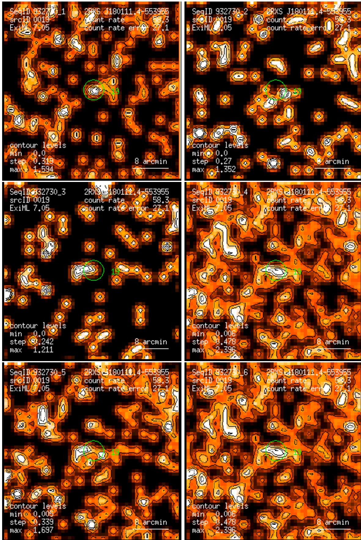
Figure 19: RASS 932730: detection 0019: band rate images, Gaussian filter: (1) PSPC channels 11 – 41, (2) 52 – 90, (3) 91 – 201, (4) 11 – 235, (5) 52 – 201, (6) 11 – 201. Broad band rates in counts/ks. Band rate contour levels in counts/ks/arcmin 2 .
