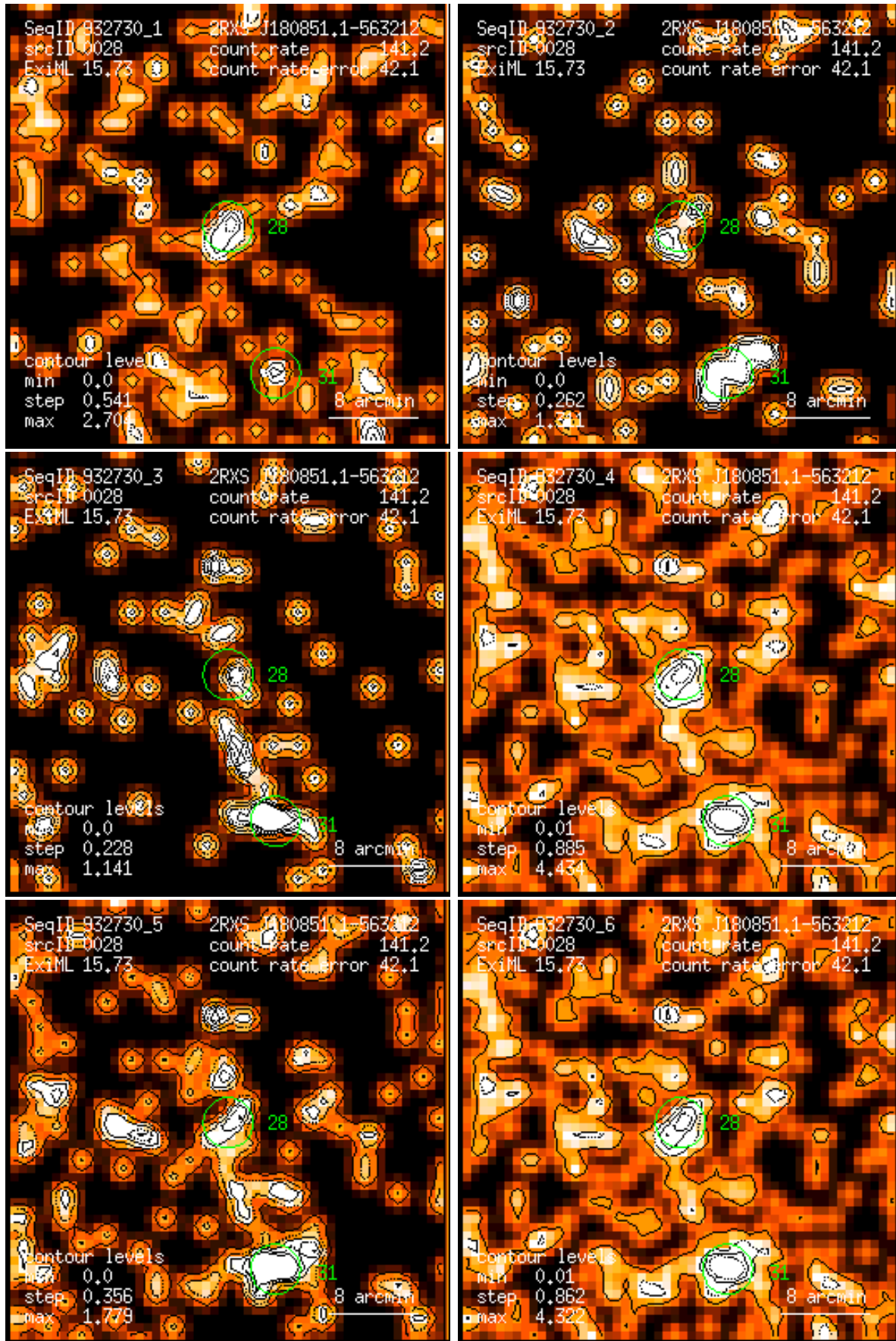
Figure 28: RASS 932730: detection 0028: band rate images, Gaussian filter: (1) PSPC channels 11 – 41, (2) 52 – 90, (3) 91 – 201, (4) 11 – 235, (5) 52 – 201, (6) 11 – 201. Broad band rates in counts/ks. Band rate contour levels in counts/ks/arcmin 2 .
