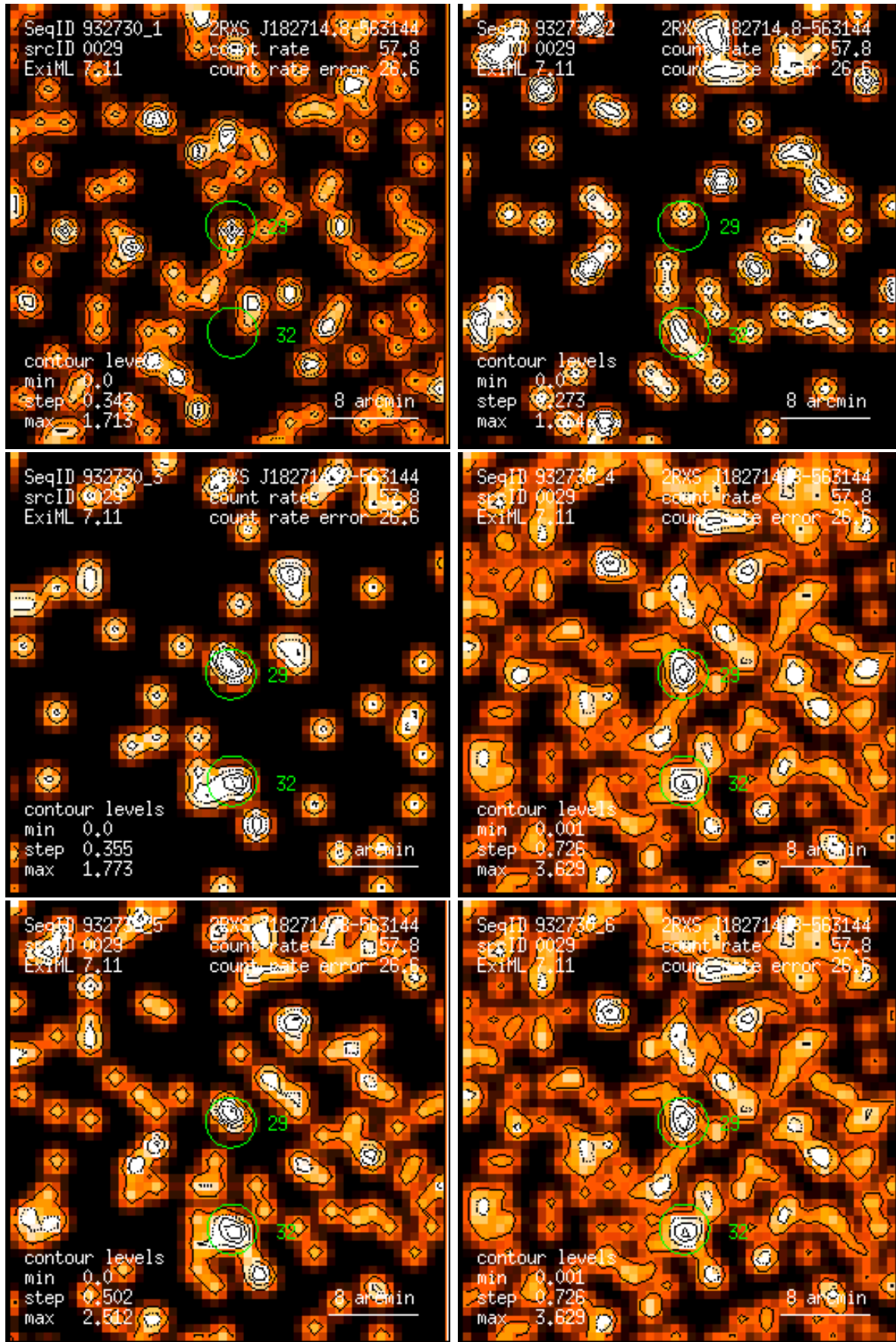
Figure 29: RASS 932730: detection 0029: band rate images, Gaussian filter: (1) PSPC channels 11 – 41, (2) 52 – 90, (3) 91 – 201, (4) 11 – 235, (5) 52 – 201, (6) 11 – 201. Broad band rates in counts/ks. Band rate contour levels in counts/ks/arcmin 2 .
