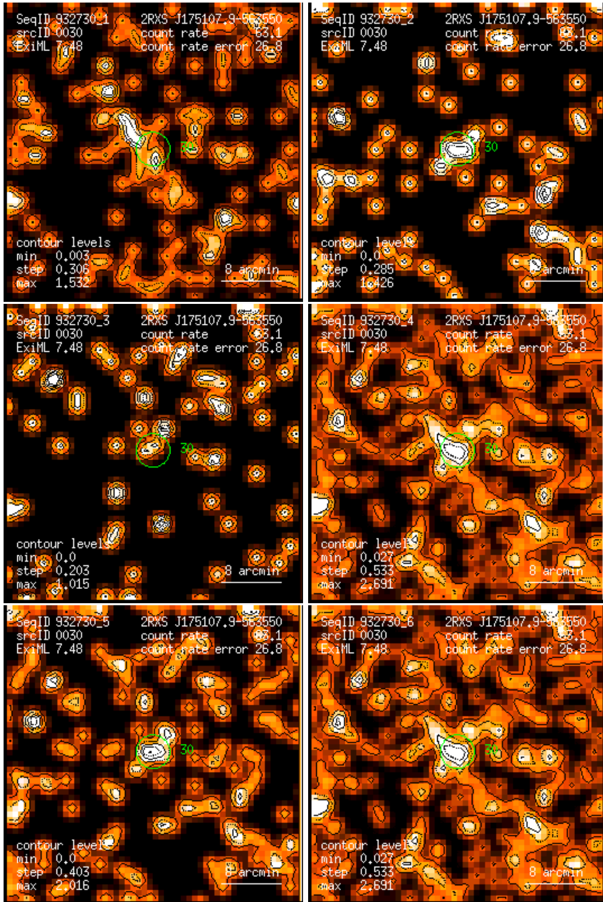
Figure 30: RASS 932730: detection 0030: band rate images, Gaussian filter: (1) PSPC channels 11 – 41, (2) 52 – 90, (3) 91 – 201, (4) 11 – 235, (5) 52 – 201, (6) 11 – 201. Broad band rates in counts/ks. Band rate contour levels in counts/ks/arcmin 2 .
