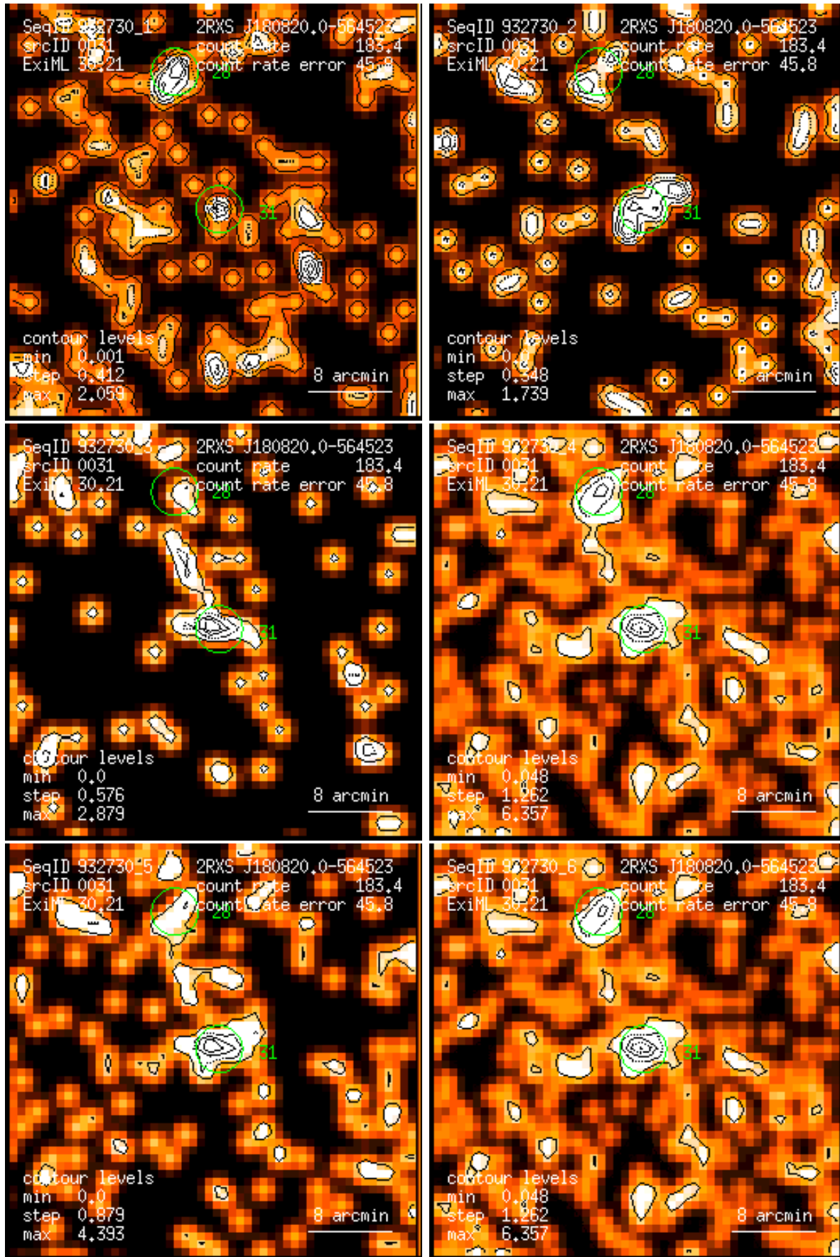
Figure 31: RASS 932730: detection 0031: band rate images, Gaussian filter: (1) PSPC channels 11 – 41, (2) 52 – 90, (3) 91 – 201, (4) 11 – 235, (5) 52 – 201, (6) 11 – 201. Broad band rates in counts/ks. Band rate contour levels in counts/ks/arcmin 2 .
