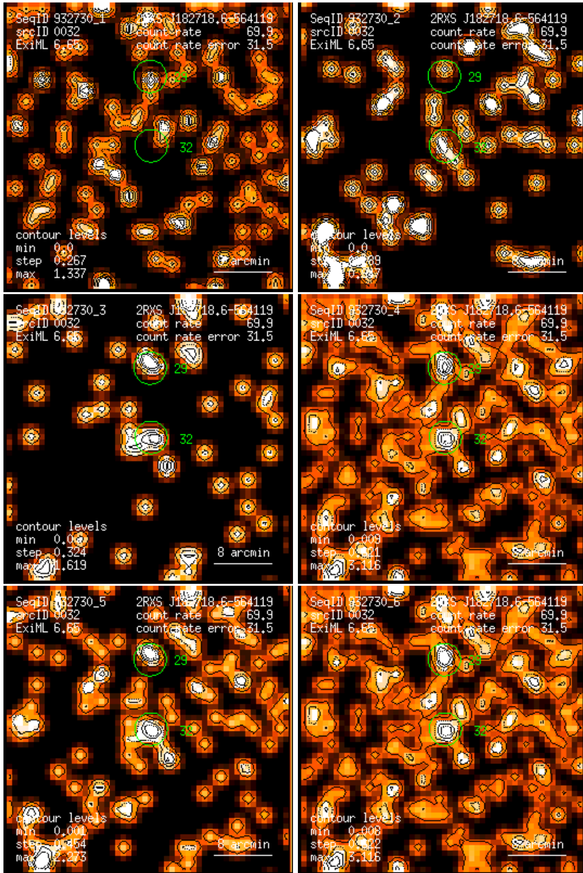
Figure 32: RASS 932730: detection 0032: band rate images, Gaussian filter: (1) PSPC channels 11 – 41, (2) 52 – 90, (3) 91 – 201, (4) 11 – 235, (5) 52 – 201, (6) 11 – 201. Broad band rates in counts/ks. Band rate contour levels in counts/ks/arcmin 2 .
