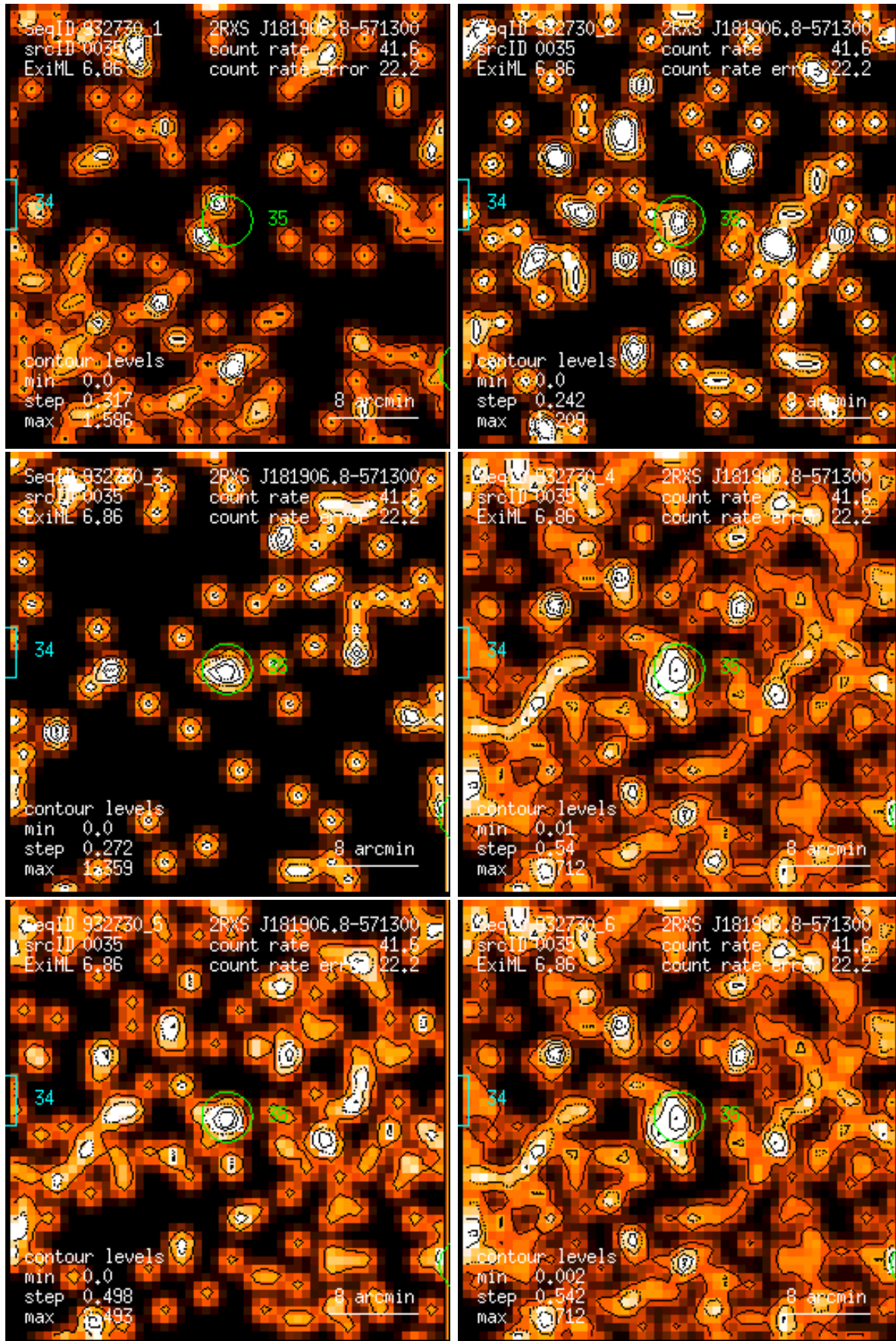
Figure 35: RASS 932730: detection 0035: band rate images, Gaussian filter: (1) PSPC channels 11 – 41, (2) 52 – 90, (3) 91 – 201, (4) 11 – 235, (5) 52 – 201, (6) 11 – 201. Broad band rates in counts/ks. Band rate contour levels in counts/ks/arcmin 2 .
