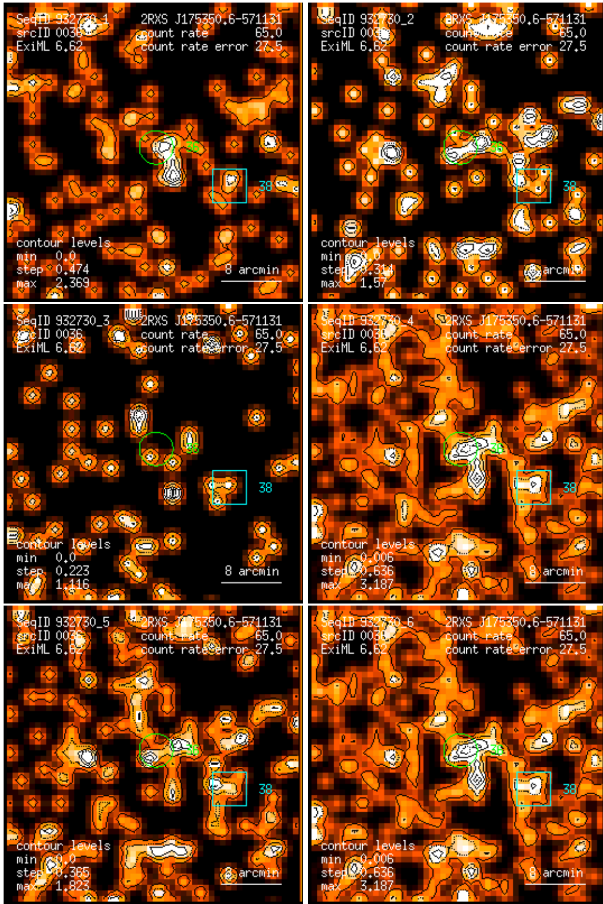
Figure 36: RASS 932730: detection 0036: band rate images, Gaussian filter: (1) PSPC channels 11 – 41, (2) 52 – 90, (3) 91 – 201, (4) 11 – 235, (5) 52 – 201, (6) 11 – 201. Broad band rates in counts/ks. Band rate contour levels in counts/ks/arcmin 2 .
