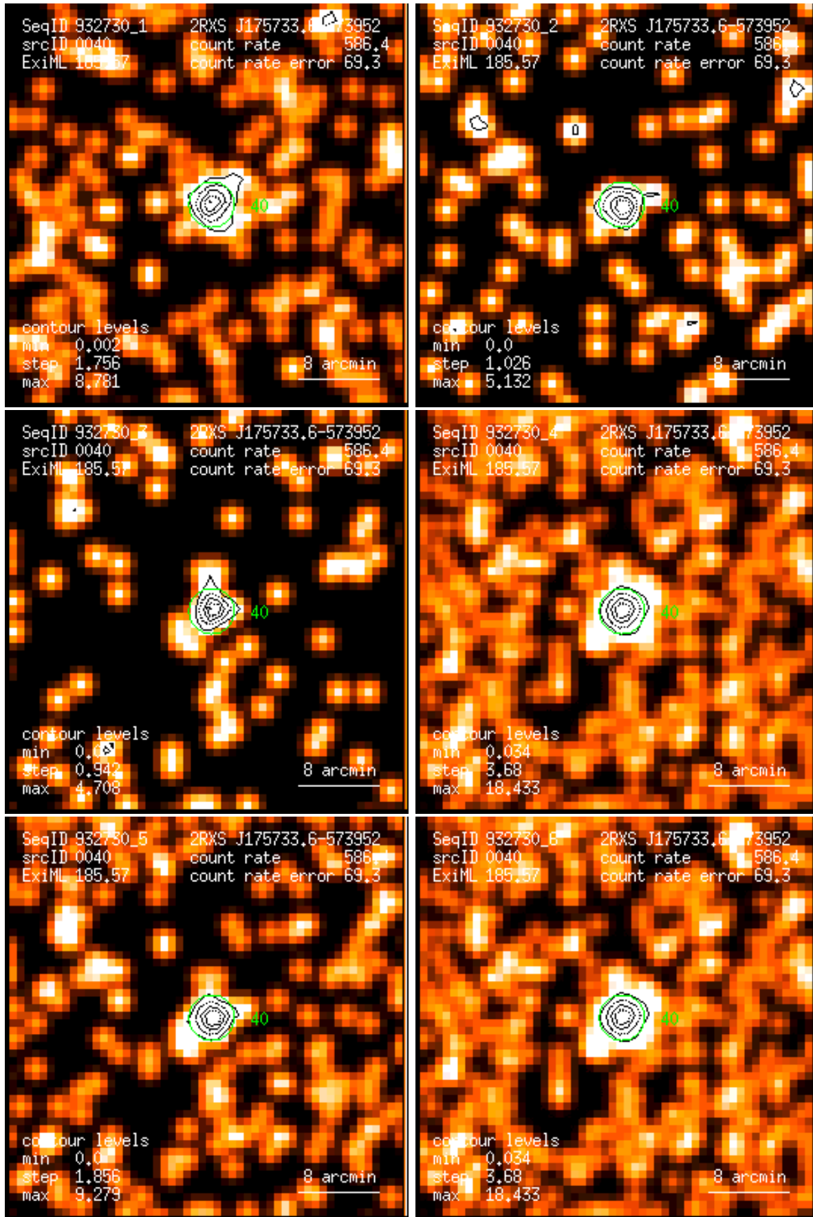
Figure 40: RASS 932730: detection 0040: band rate images, Gaussian filter: (1) PSPC channels 11 – 41, (2) 52 – 90, (3) 91 – 201, (4) 11 – 235, (5) 52 – 201, (6) 11 – 201. Broad band rates in counts/ks. Band rate contour levels in counts/ks/arcmin 2 .
