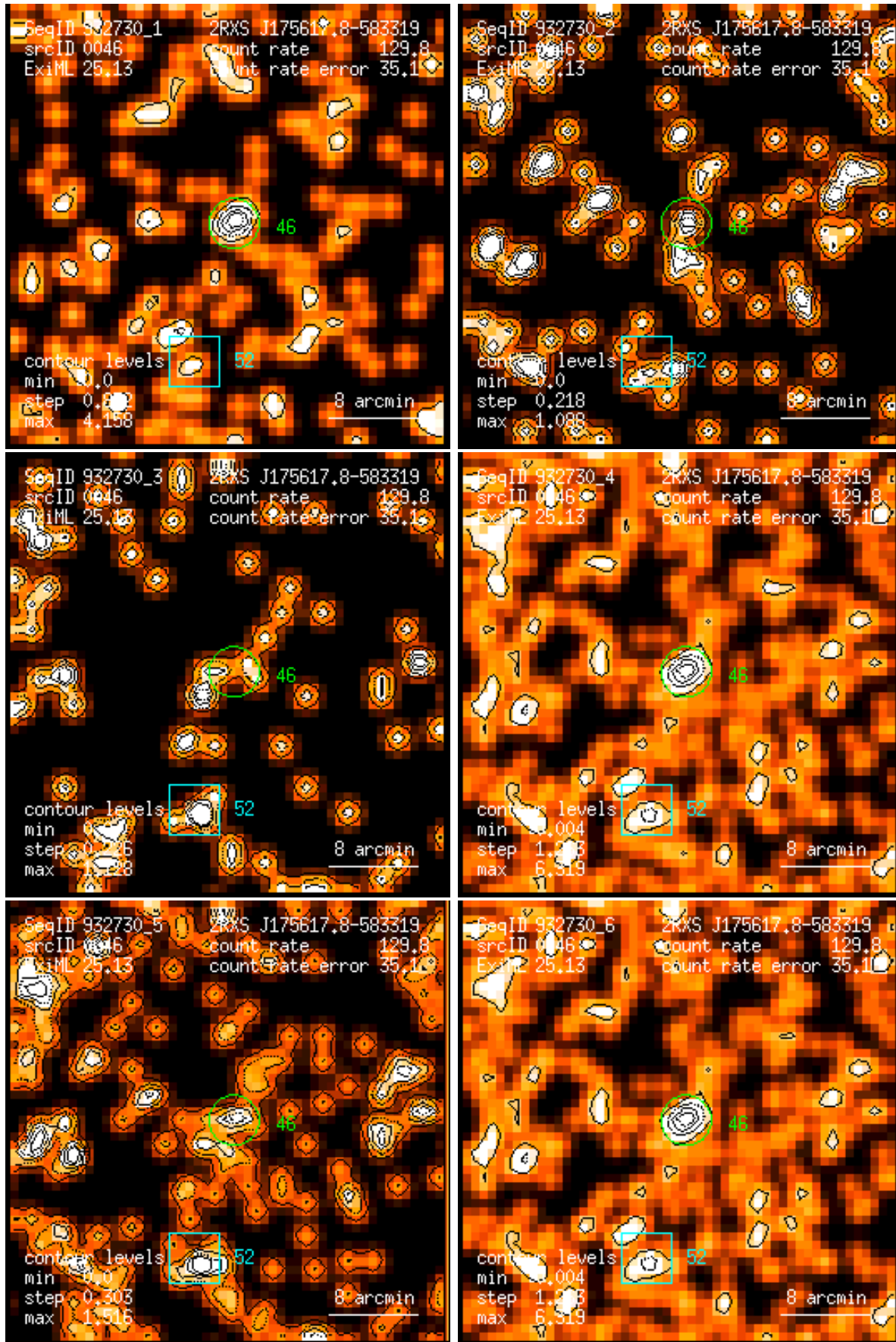
Figure 46: RASS 932730: detection 0046: band rate images, Gaussian filter: (1) PSPC channels 11 – 41, (2) 52 – 90, (3) 91 – 201, (4) 11 – 235, (5) 52 – 201, (6) 11 – 201. Broad band rates in counts/ks. Band rate contour levels in counts/ks/arcmin 2 .
