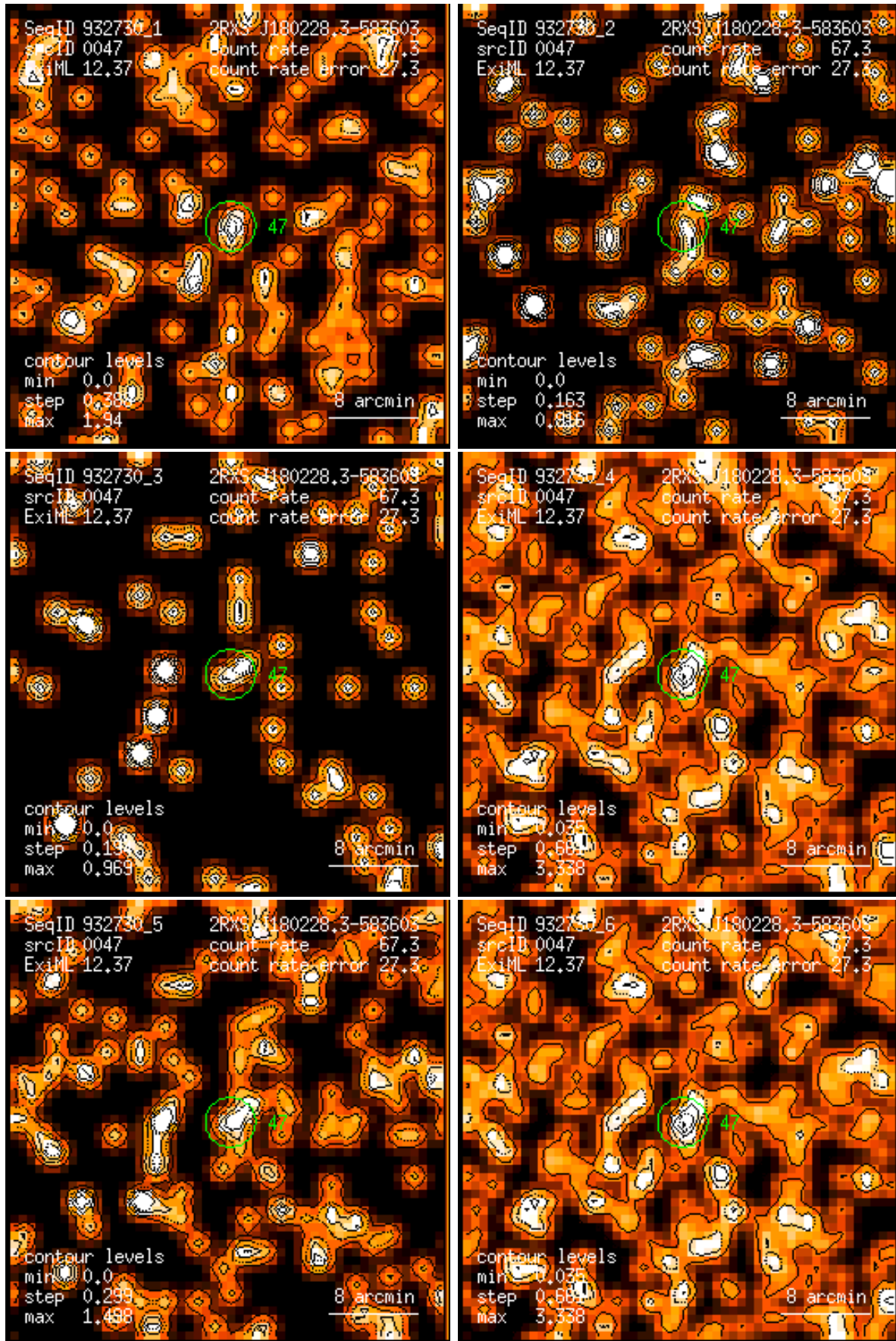
Figure 47: RASS 932730: detection 0047: band rate images, Gaussian filter: (1) PSPC channels 11 – 41, (2) 52 – 90, (3) 91 – 201, (4) 11 – 235, (5) 52 – 201, (6) 11 – 201. Broad band rates in counts/ks. Band rate contour levels in counts/ks/arcmin 2 .
