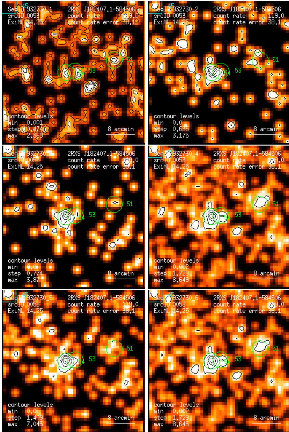
Figure 53: RASS 932730: detection 0053: band rate images, Gaussian filter: (1) PSPC channels 11 – 41, (2) 52 – 90, (3) 91 – 201, (4) 11 – 235, (5) 52 – 201, (6) 11 – 201. Broad band rates in counts/ks. Band rate contour levels in counts/ks/arcmin 2 .
