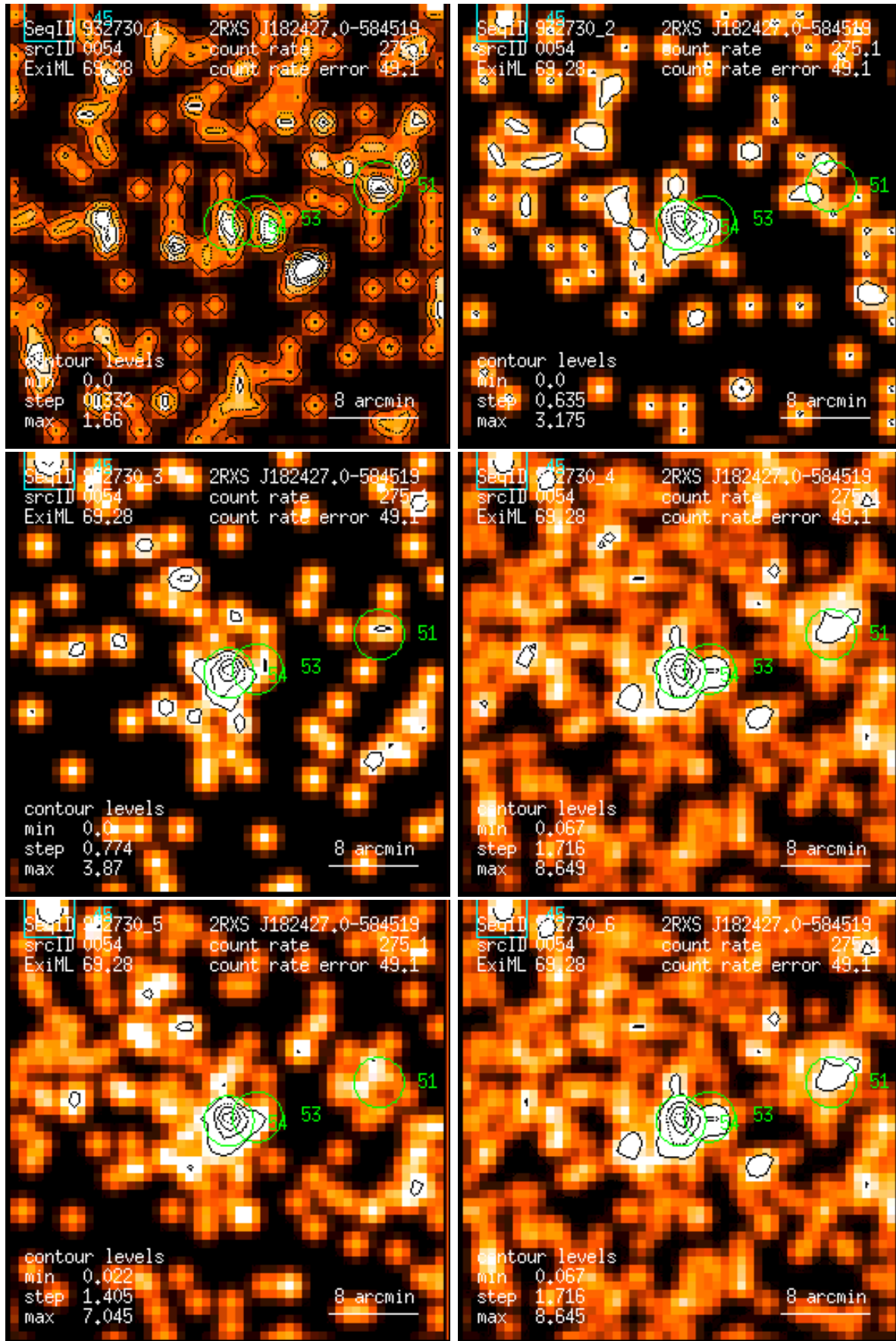
Figure 54: RASS 932730: detection 0054: band rate images, Gaussian filter: (1) PSPC channels 11 – 41, (2) 52 – 90, (3) 91 – 201, (4) 11 – 235, (5) 52 – 201, (6) 11 – 201. Broad band rates in counts/ks. Band rate contour levels in counts/ks/arcmin 2 .
