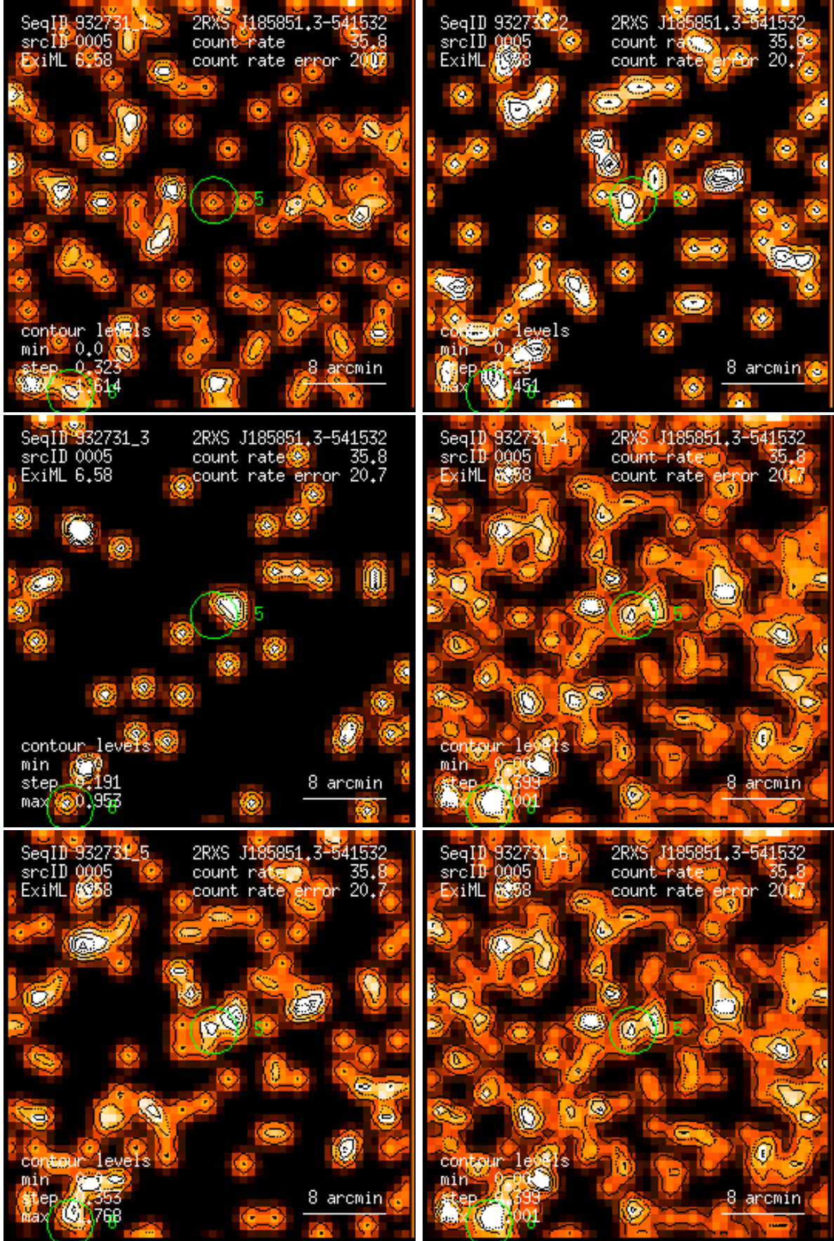
Figure 5: RASS 932731: detection 0005: band rate images, Gaussian filter: (1) PSPC channels 11 – 41, (2) 52 – 90, (3) 91 – 201, (4) 11 – 235, (5) 52 – 201, (6) 11 – 201. Broad band rates in counts/ks. Band rate contour levels in counts/ks/arcmin 2 .
