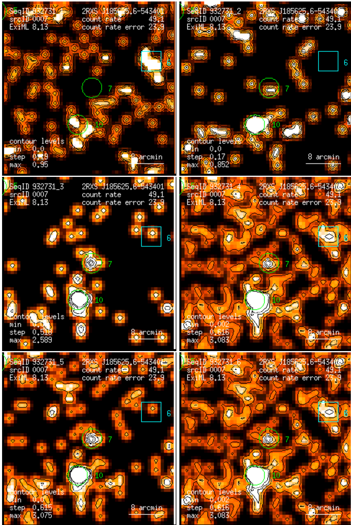
Figure 7: RASS 932731: detection 0007: band rate images, Gaussian filter: (1) PSPC channels 11 – 41, (2) 52 – 90, (3) 91 – 201, (4) 11 – 235, (5) 52 – 201, (6) 11 – 201. Broad band rates in counts/ks. Band rate contour levels in counts/ks/arcmin 2 .
