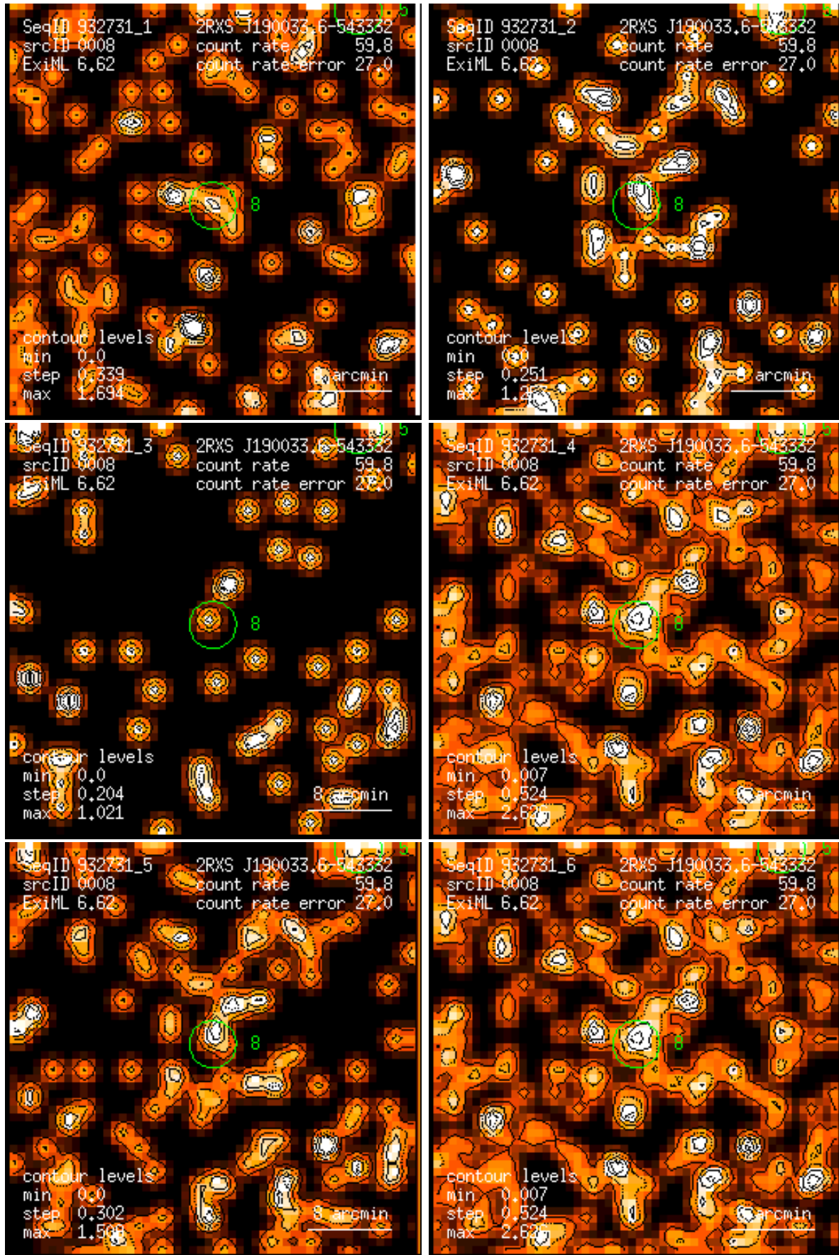
Figure 8: RASS 932731: detection 0008: band rate images, Gaussian filter: (1) PSPC channels 11 – 41, (2) 52 – 90, (3) 91 – 201, (4) 11 – 235, (5) 52 – 201, (6) 11 – 201. Broad band rates in counts/ks. Band rate contour levels in counts/ks/arcmin 2 .
