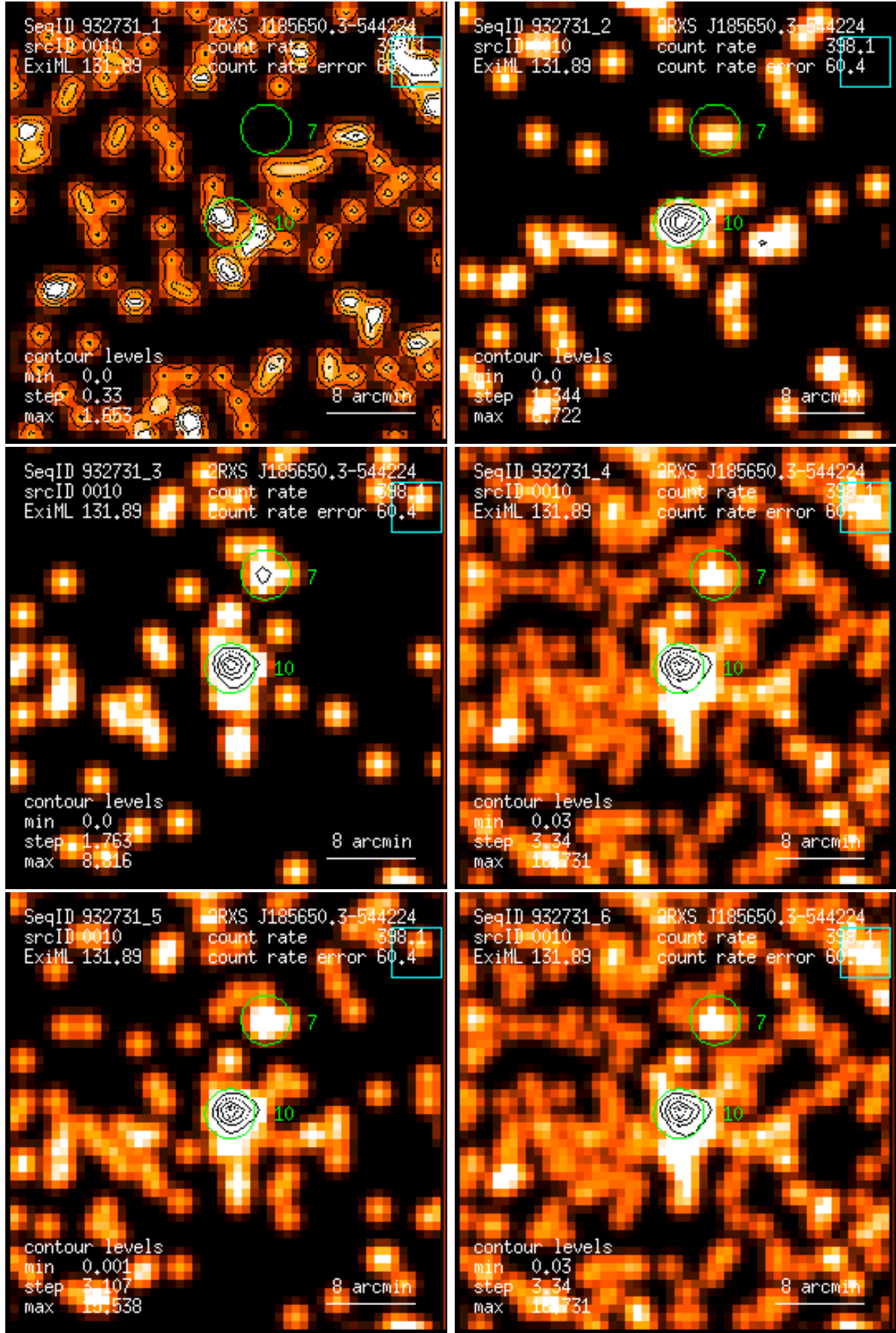
Figure 10: RASS 932731: detection 0010: band rate images, Gaussian filter: (1) PSPC channels 11 – 41, (2) 52 – 90, (3) 91 – 201, (4) 11 – 235, (5) 52 – 201, (6) 11 – 201. Broad band rates in counts/ks. Band rate contour levels in counts/ks/arcmin 2 .
