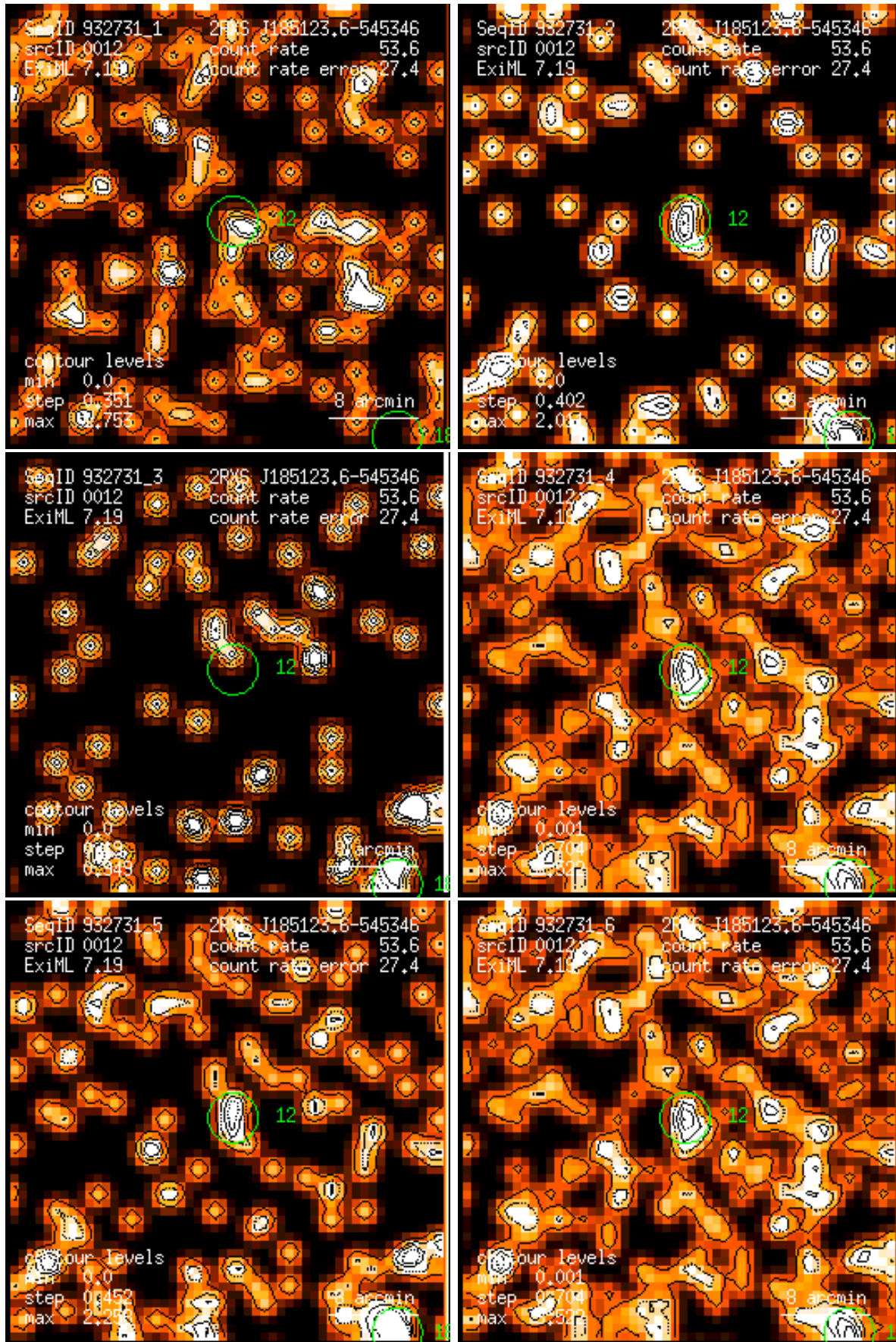
Figure 12: RASS 932731: detection 0012: band rate images, Gaussian filter: (1) PSPC channels 11 – 41, (2) 52 – 90, (3) 91 – 201, (4) 11 – 235, (5) 52 – 201, (6) 11 – 201. Broad band rates in counts/ks. Band rate contour levels in counts/ks/arcmin 2 .
