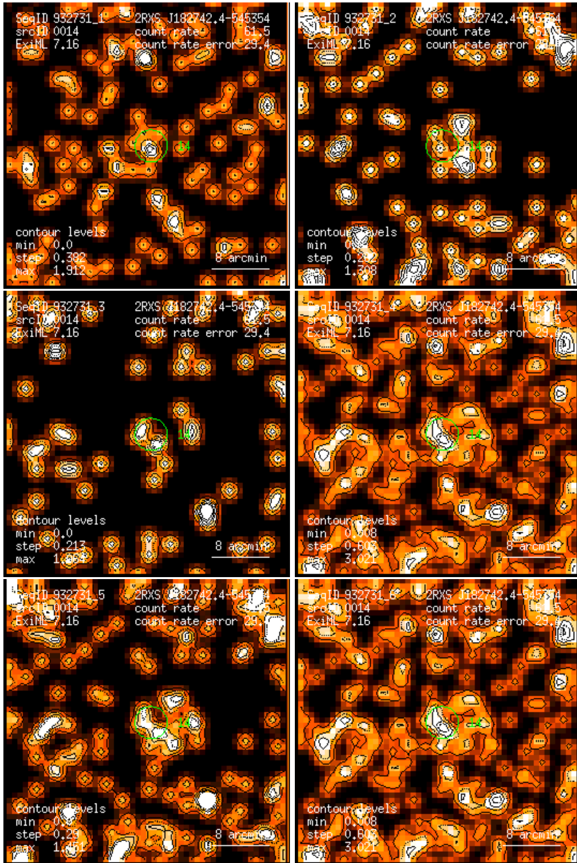
Figure 14: RASS 932731: detection 0014: band rate images, Gaussian filter: (1) PSPC channels 11 – 41, (2) 52 – 90, (3) 91 – 201, (4) 11 – 235, (5) 52 – 201, (6) 11 – 201. Broad band rates in counts/ks. Band rate contour levels in counts/ks/arcmin 2 .
