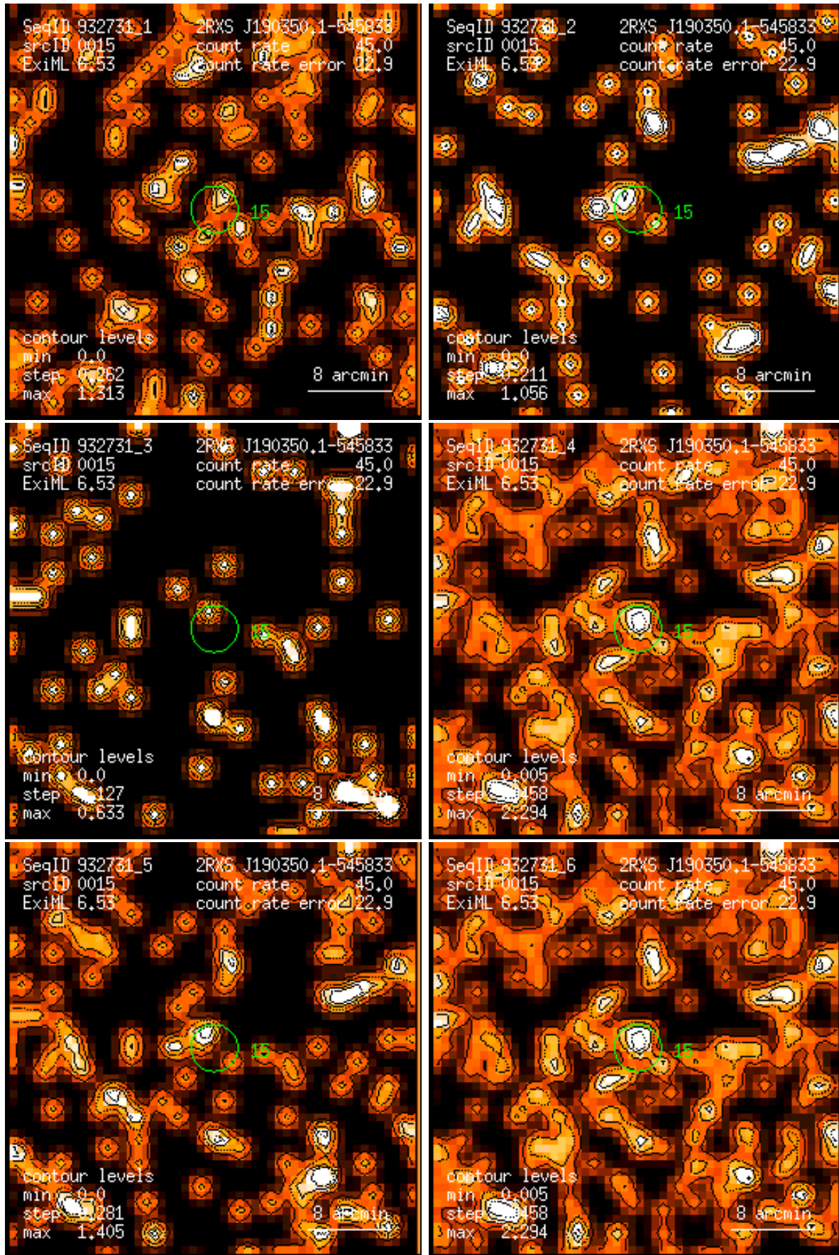
Figure 15: RASS 932731: detection 0015: band rate images, Gaussian filter: (1) PSPC channels 11 – 41, (2) 52 – 90, (3) 91 – 201, (4) 11 – 235, (5) 52 – 201, (6) 11 – 201. Broad band rates in counts/ks. Band rate contour levels in counts/ks/arcmin 2 .
