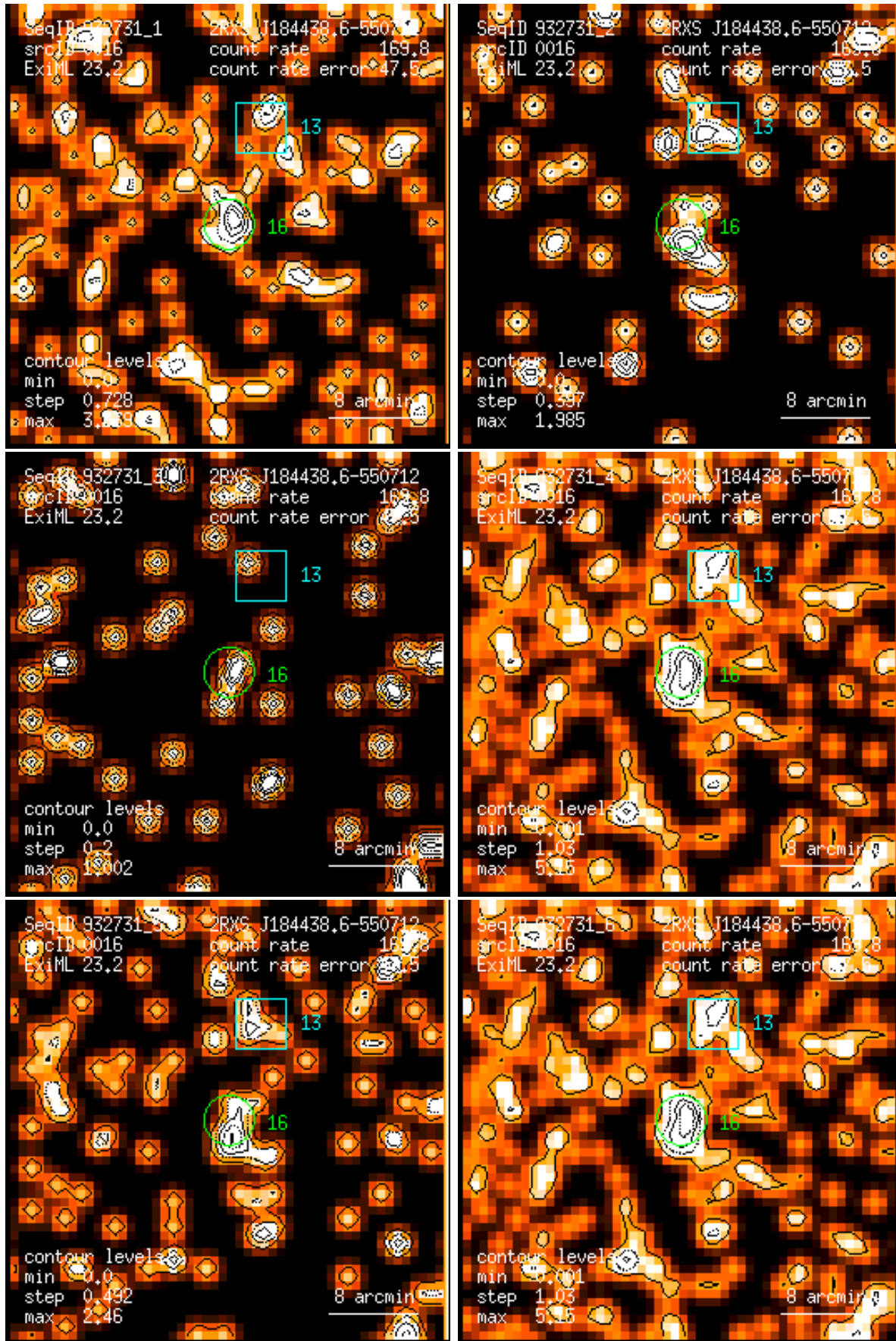
Figure 16: RASS 932731: detection 0016: band rate images, Gaussian filter: (1) PSPC channels 11 – 41, (2) 52 – 90, (3) 91 – 201, (4) 11 – 235, (5) 52 – 201, (6) 11 – 201. Broad band rates in counts/ks. Band rate contour levels in counts/ks/arcmin 2 .
