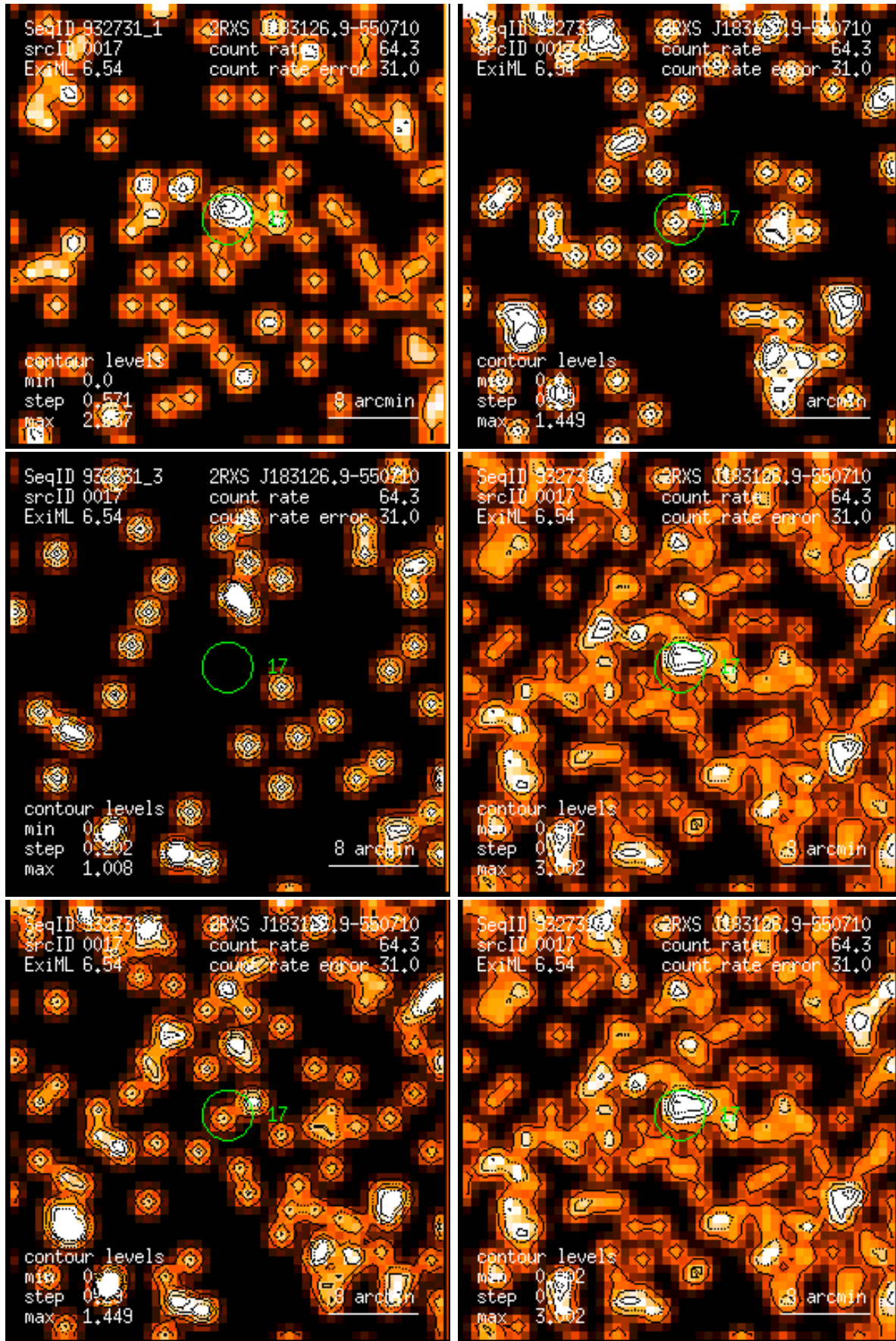
Figure 17: RASS 932731: detection 0017: band rate images, Gaussian filter: (1) PSPC channels 11 – 41, (2) 52 – 90, (3) 91 – 201, (4) 11 – 235, (5) 52 – 201, (6) 11 – 201. Broad band rates in counts/ks. Band rate contour levels in counts/ks/arcmin 2 .
