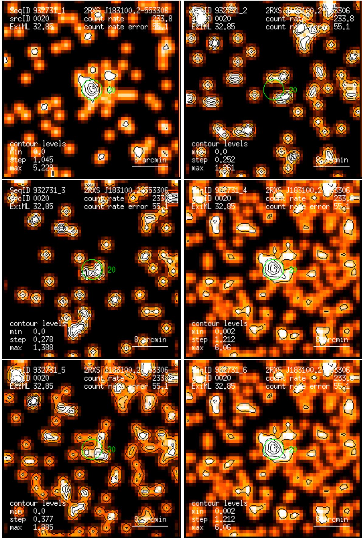
Figure 20: RASS 932731: detection 0020: band rate images, Gaussian filter: (1) PSPC channels 11 – 41, (2) 52 – 90, (3) 91 – 201, (4) 11 – 235, (5) 52 – 201, (6) 11 – 201. Broad band rates in counts/ks. Band rate contour levels in counts/ks/arcmin 2 .
