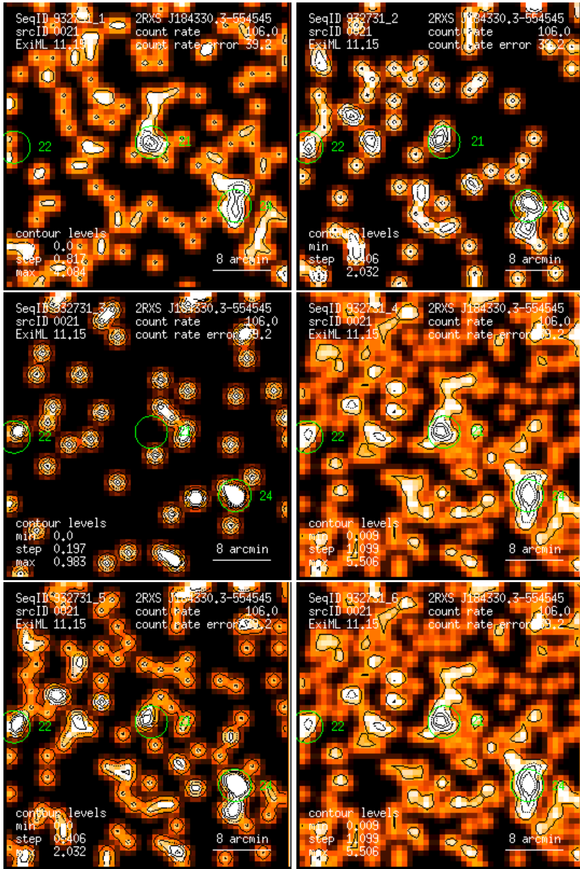
Figure 21: RASS 932731: detection 0021: band rate images, Gaussian filter: (1) PSPC channels 11 – 41, (2) 52 – 90, (3) 91 – 201, (4) 11 – 235, (5) 52 – 201, (6) 11 – 201. Broad band rates in counts/ks. Band rate contour levels in counts/ks/arcmin 2 .
