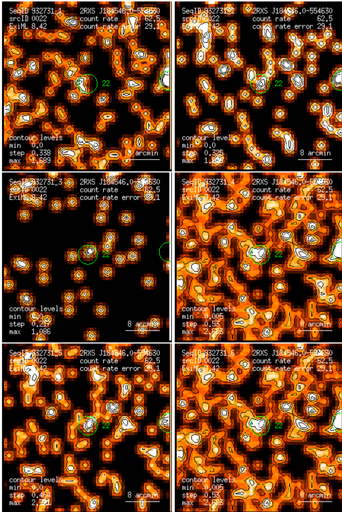
Figure 22: RASS 932731: detection 0022: band rate images, Gaussian filter: (1) PSPC channels 11 – 41, (2) 52 – 90, (3) 91 – 201, (4) 11 – 235, (5) 52 – 201, (6) 11 – 201. Broad band rates in counts/ks. Band rate contour levels in counts/ks/arcmin 2 .
