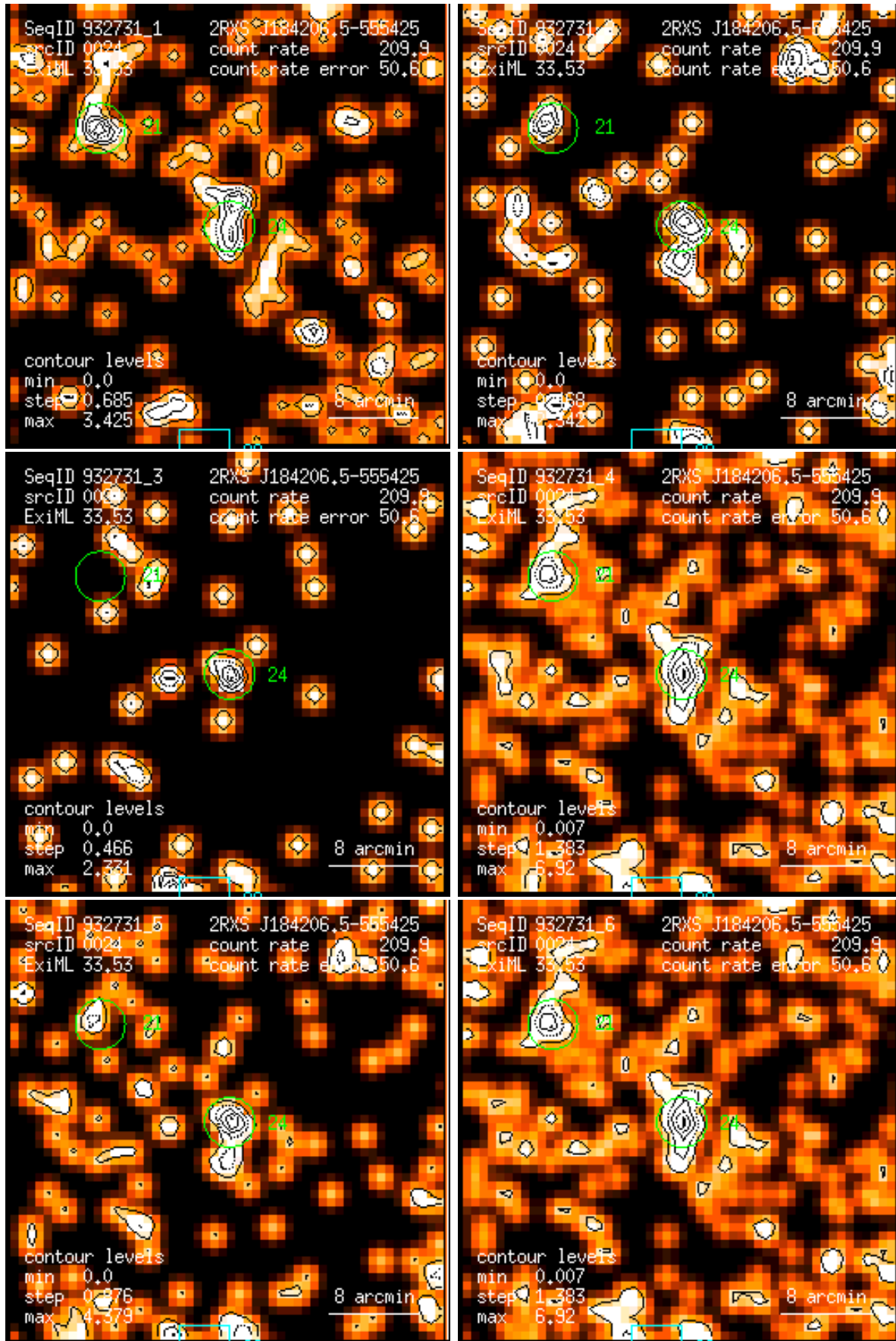
Figure 24: RASS 932731: detection 0024: band rate images, Gaussian filter: (1) PSPC channels 11 – 41, (2) 52 – 90, (3) 91 – 201, (4) 11 – 235, (5) 52 – 201, (6) 11 – 201. Broad band rates in counts/ks. Band rate contour levels in counts/ks/arcmin 2 .
