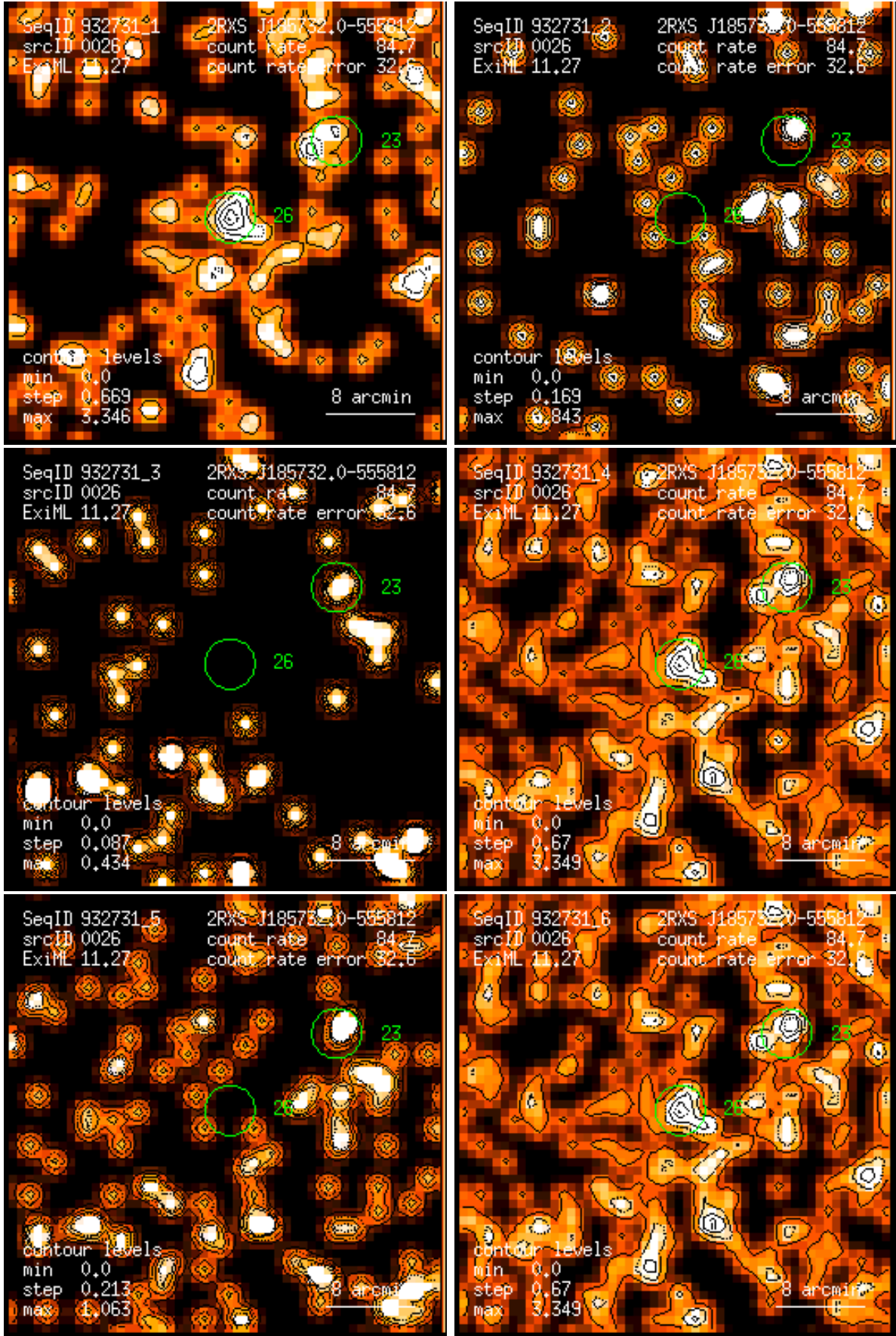
Figure 26: RASS 932731: detection 0026: band rate images, Gaussian filter: (1) PSPC channels 11 – 41, (2) 52 – 90, (3) 91 – 201, (4) 11 – 235, (5) 52 – 201, (6) 11 – 201. Broad band rates in counts/ks. Band rate contour levels in counts/ks/arcmin 2 .
