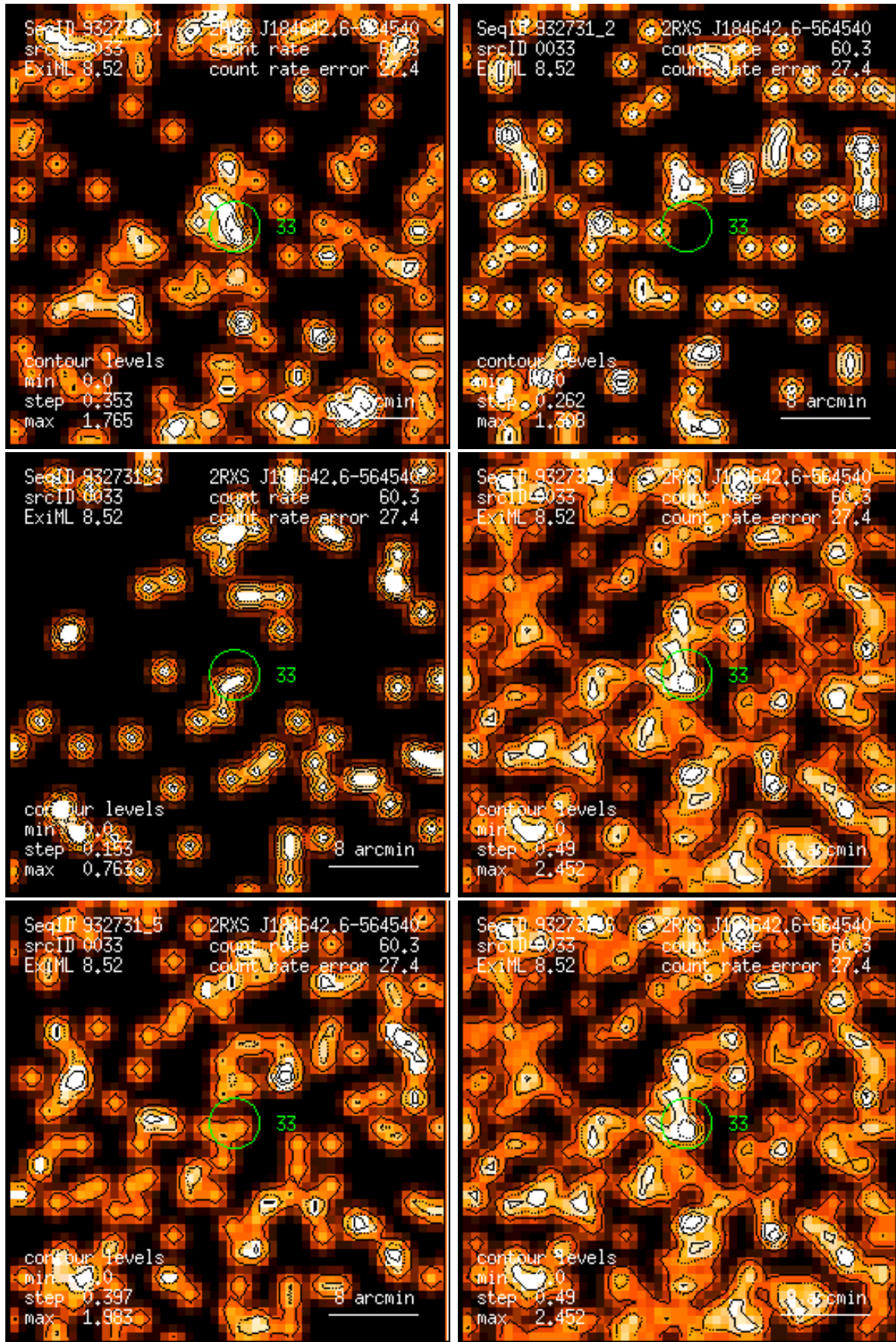
Figure 33: RASS 932731: detection 0033: band rate images, Gaussian filter: (1) PSPC channels 11 – 41, (2) 52 – 90, (3) 91 – 201, (4) 11 – 235, (5) 52 – 201, (6) 11 – 201. Broad band rates in counts/ks. Band rate contour levels in counts/ks/arcmin 2 .
