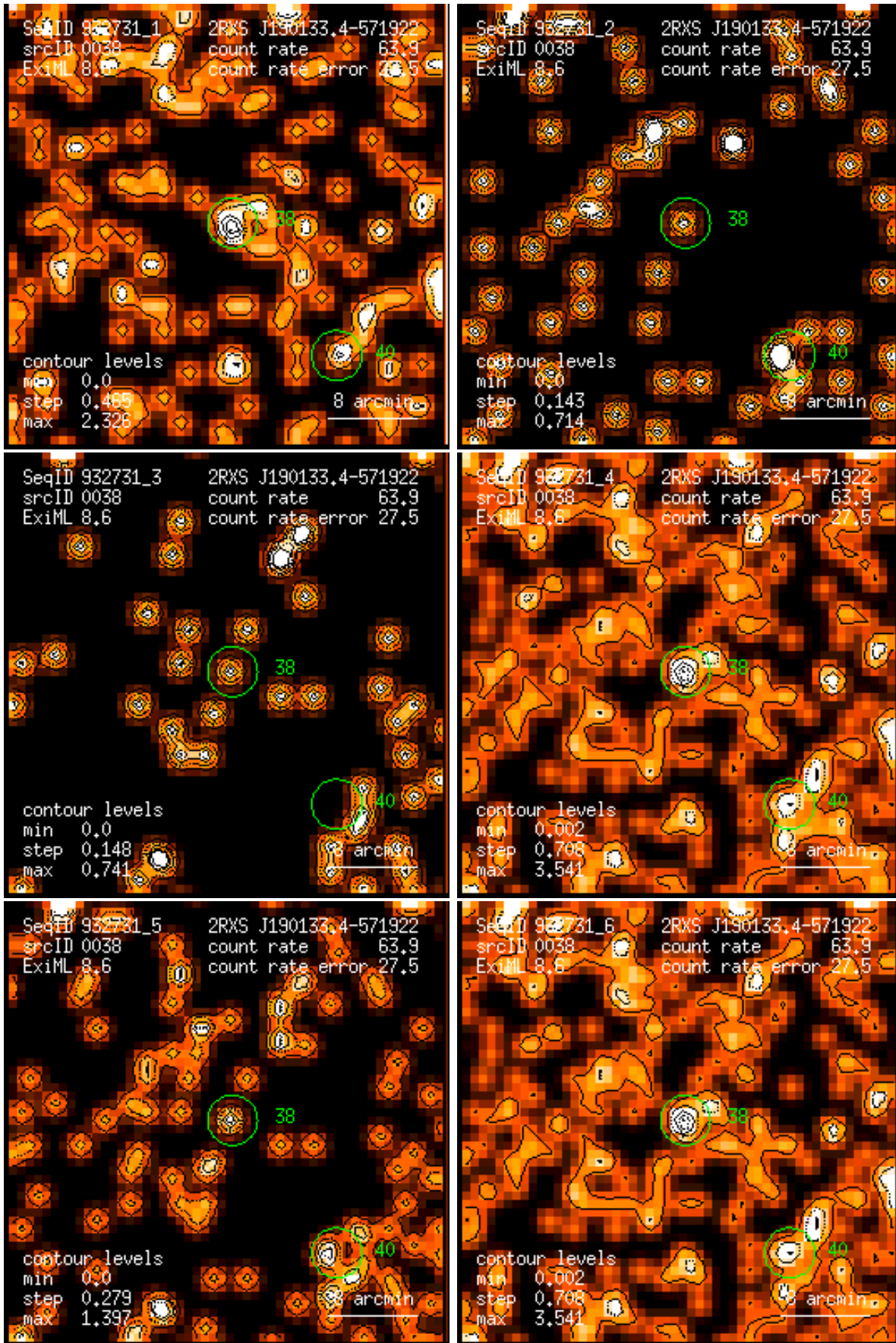
Figure 38: RASS 932731: detection 0038: band rate images, Gaussian filter: (1) PSPC channels 11 – 41, (2) 52 – 90, (3) 91 – 201, (4) 11 – 235, (5) 52 – 201, (6) 11 – 201. Broad band rates in counts/ks. Band rate contour levels in counts/ks/arcmin 2 .
