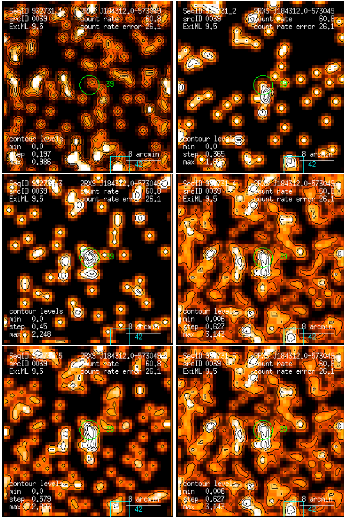
Figure 39: RASS 932731: detection 0039: band rate images, Gaussian filter: (1) PSPC channels 11 – 41, (2) 52 – 90, (3) 91 – 201, (4) 11 – 235, (5) 52 – 201, (6) 11 – 201. Broad band rates in counts/ks. Band rate contour levels in counts/ks/arcmin 2 .
