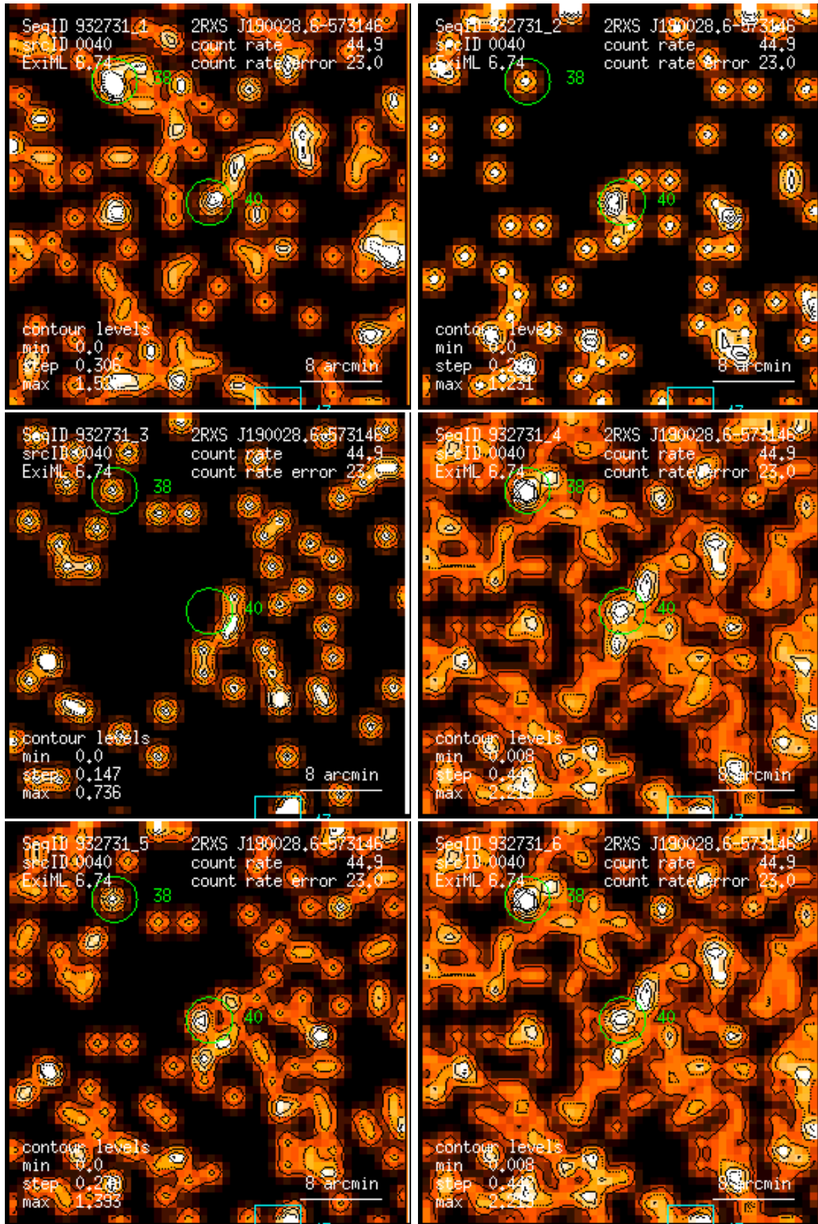
Figure 40: RASS 932731: detection 0040: band rate images, Gaussian filter: (1) PSPC channels 11 – 41, (2) 52 – 90, (3) 91 – 201, (4) 11 – 235, (5) 52 – 201, (6) 11 – 201. Broad band rates in counts/ks. Band rate contour levels in counts/ks/arcmin 2 .
